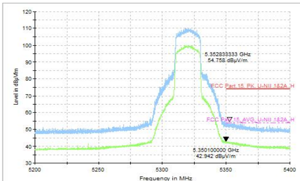
Fig. 28 Band Edges CH64 5320MHz, MIMO
