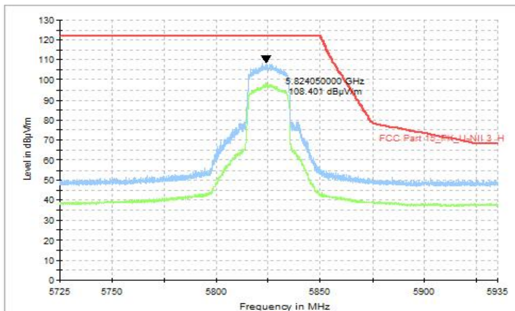
Fig. 32 Band Edges, CH165 5825MHz, MIMO
