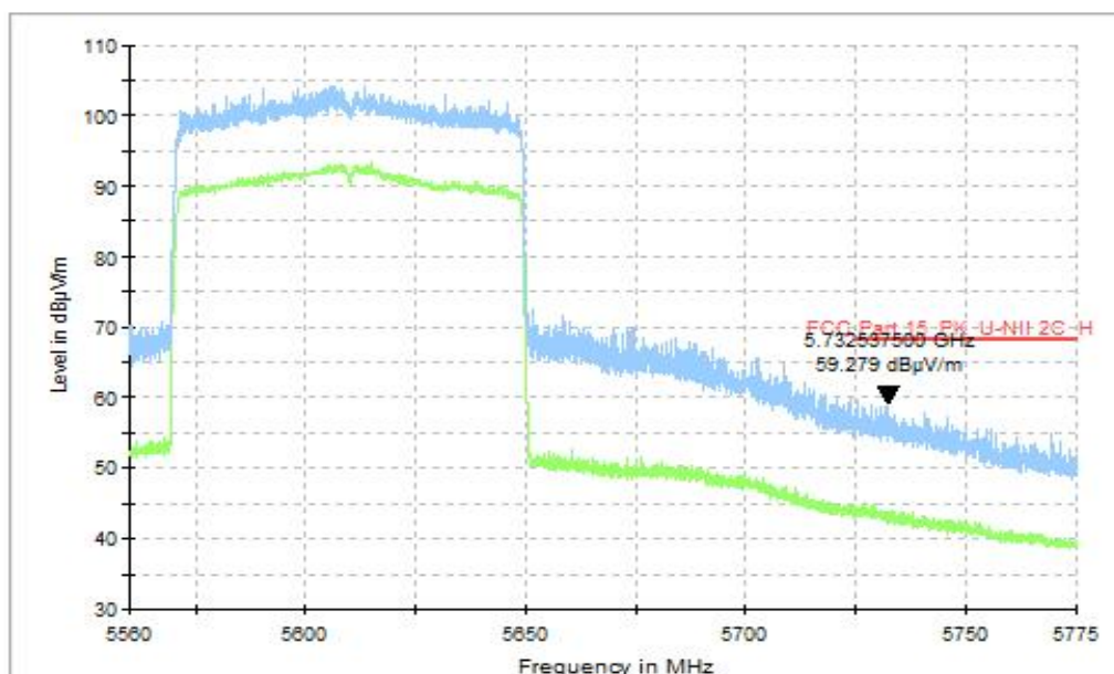
Fig. 42 Band Edges, CH122 5610MHz, MIMO
