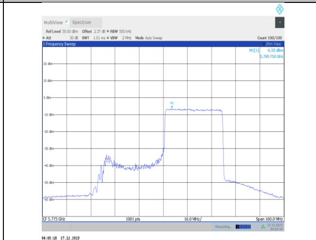
11ax80MIMO-Ant4-5775-484Tone-RU66-PASS
