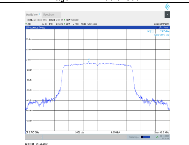
11ax20MIMO-Ant4-5745-PASS
