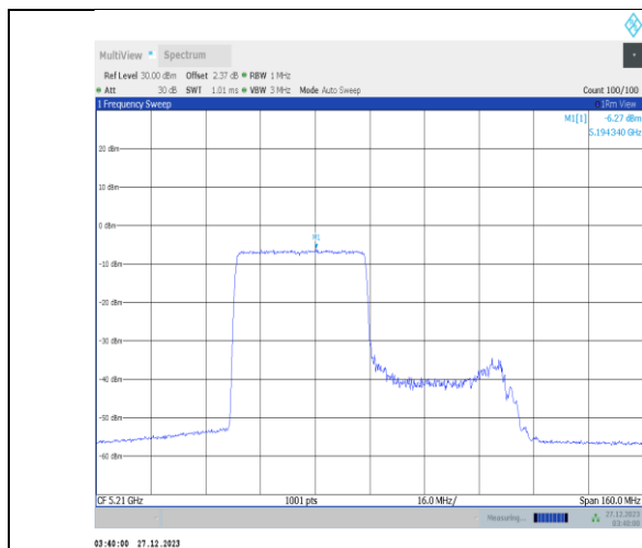
11ax80MIMO-Ant3-5210-484Tone-RU65-PASS
