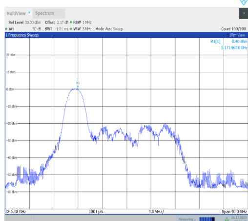
11ax20MIMO-Ant4-5180-26Tone-RU0-PASS
