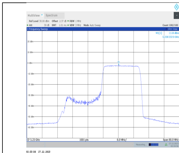
11ax40MIMO-Ant3-5230-242Tone-RU62-PASS
