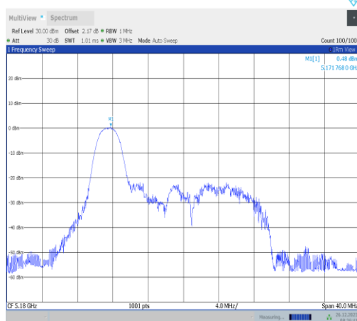
11ax20MIMO-Ant3-5180-26Tone-RU0-PASS
