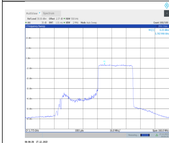
11ax80MIMO-Ant3-5775-484Tone-RU66-PASS
