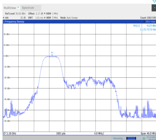
11ax20MIMO-Ant4-5180-52Tone-RU37-PASS
