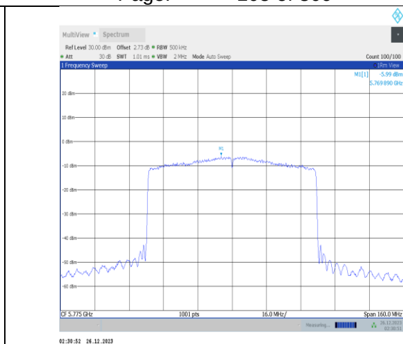
11ax80MIMO-Ant2-5775-PASS
