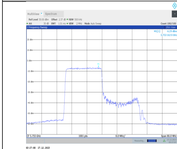
11ax40MIMO-Ant3-5755-242Tone-RU61-PASS
