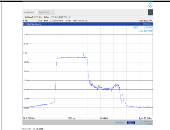
11ax40MIMO-Ant2-5755-242Tone-RU61-PASS
