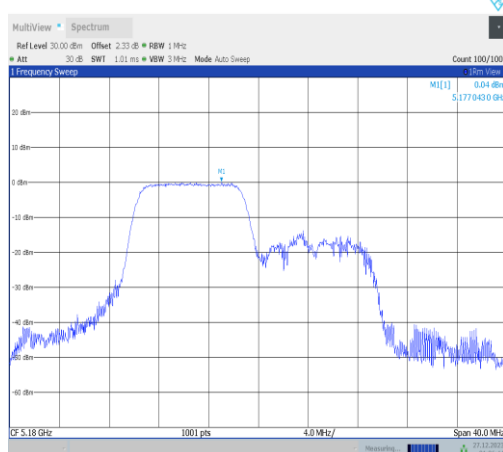
11ax20MIMO-Ant3-5180-106Tone-RU53-PASS
