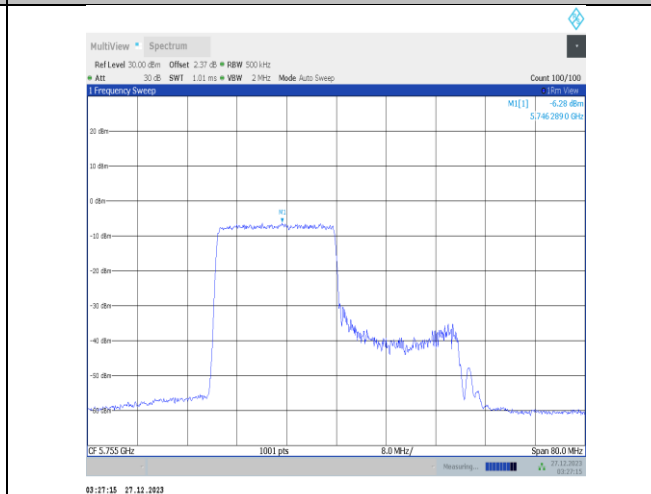
11ax40MIMO-Ant4-5755-242Tone-RU61-PASS
