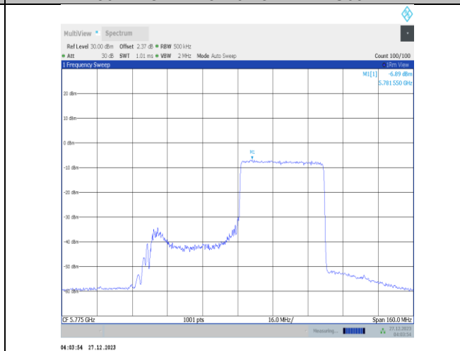
11ax80MIMO-Ant2-5775-484Tone-RU66-PASS
