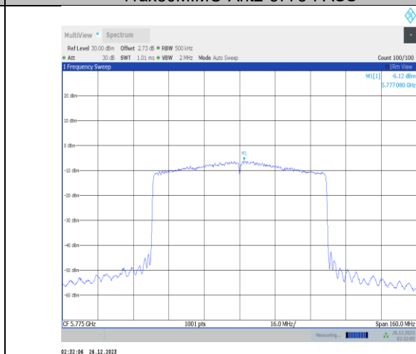
11ax80MIMO-Ant4-5775-PASS
