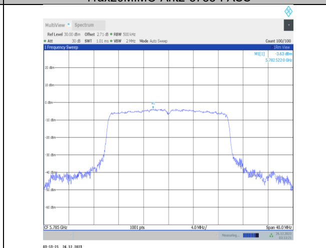
11ax20MIMO-Ant4-5785-PASS
