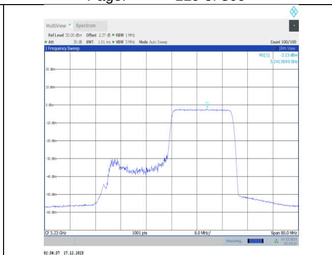
11ax40MIMO-Ant4-5230-242Tone-RU62-PASS
