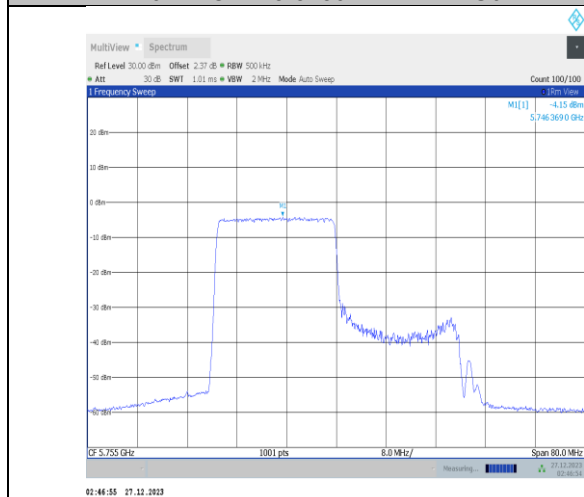
11ax40MIMO-Ant1-5755-242Tone-RU61-PASS
