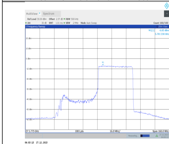
11ax80MIMO-Ant1-5775-484Tone-RU66-PASS
