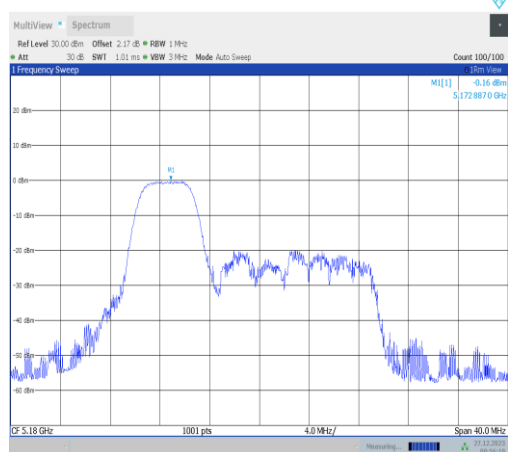
11ax20MIMO-Ant3-5180-52Tone-RU37-PASS
