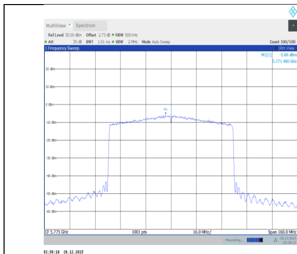
11ax80MIMO-Ant1-5775-PASS
