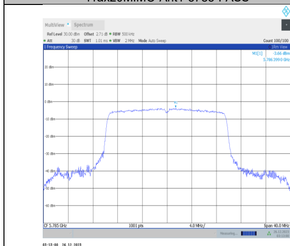
11ax20MIMO-Ant3-5785-PASS
