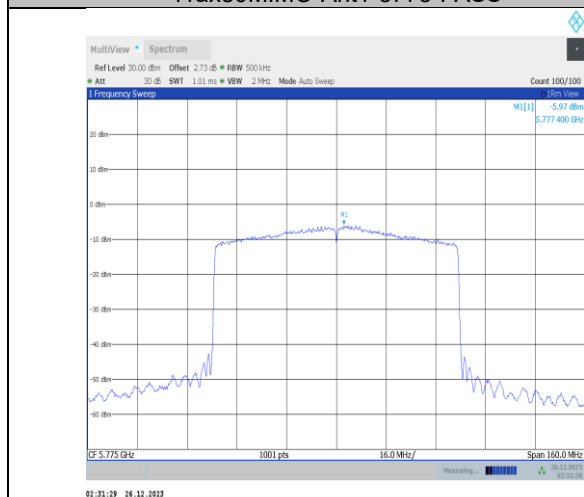
11ax80MIMO-Ant3-5775-PASS
