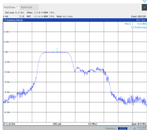
11ax20MIMO-Ant4-5180-106Tone-RU53-PASS
