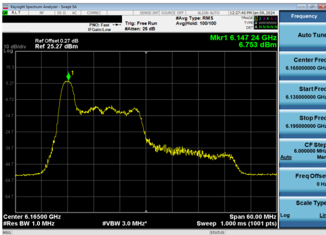
Plot 7-361. SP Power Spectral Density Plot CDD Diversity Antenna 5T (40MHz 802.11ax RU26 (UNII Band 5) – Ch. 43)
