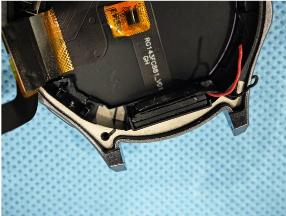
BT/Wi-Fi ANT
