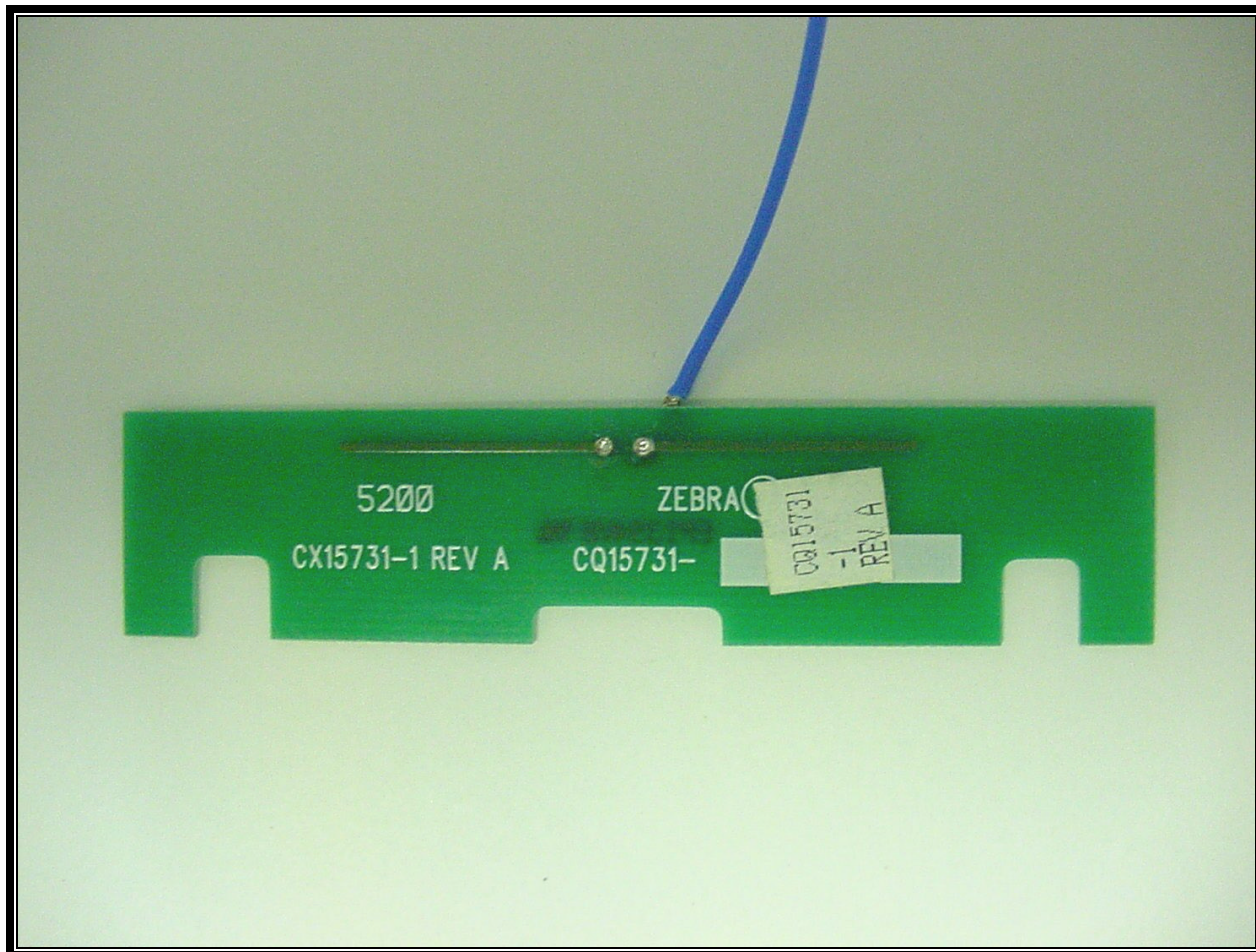
PHOTOGRAPH 37: CAMEO 2 (CQ15731-1) ANTENNA FRONT VIEW
