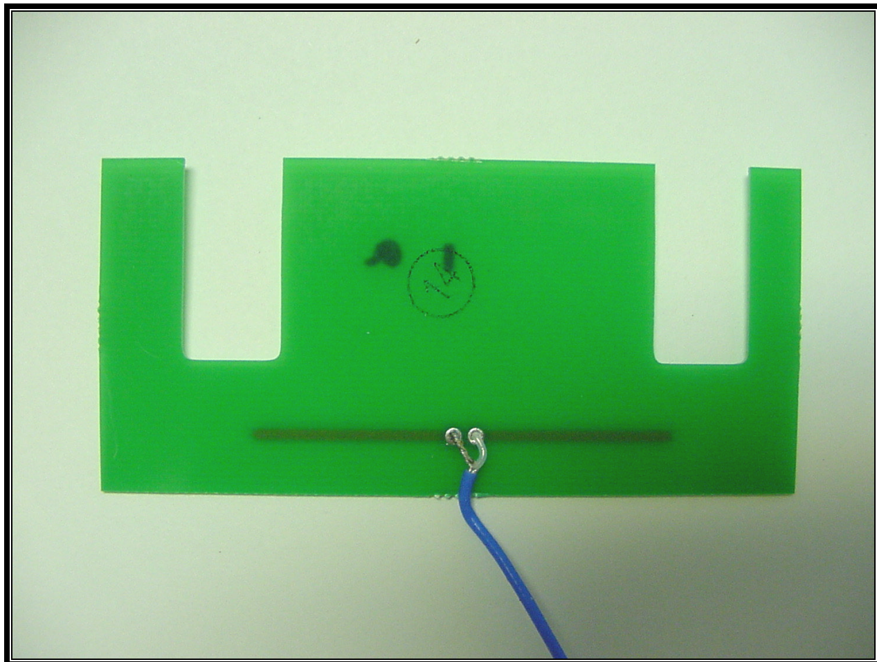
PHOTOGRAPH 36: CAMEO 3 (CQ15352-1) ANTENNA BACK VIEW
