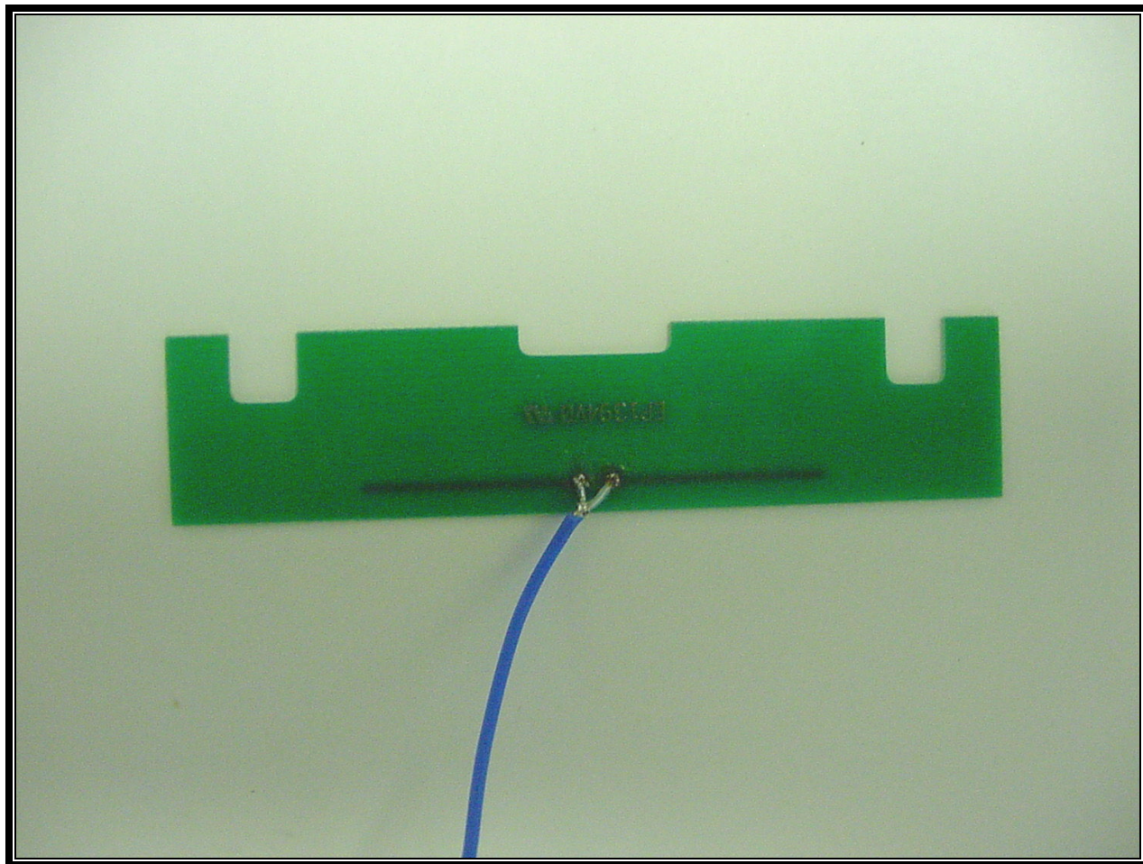
PHOTOGRAPH 38: CAME0 2 (CQ15731-1) ANTENNA BACK VIEW
