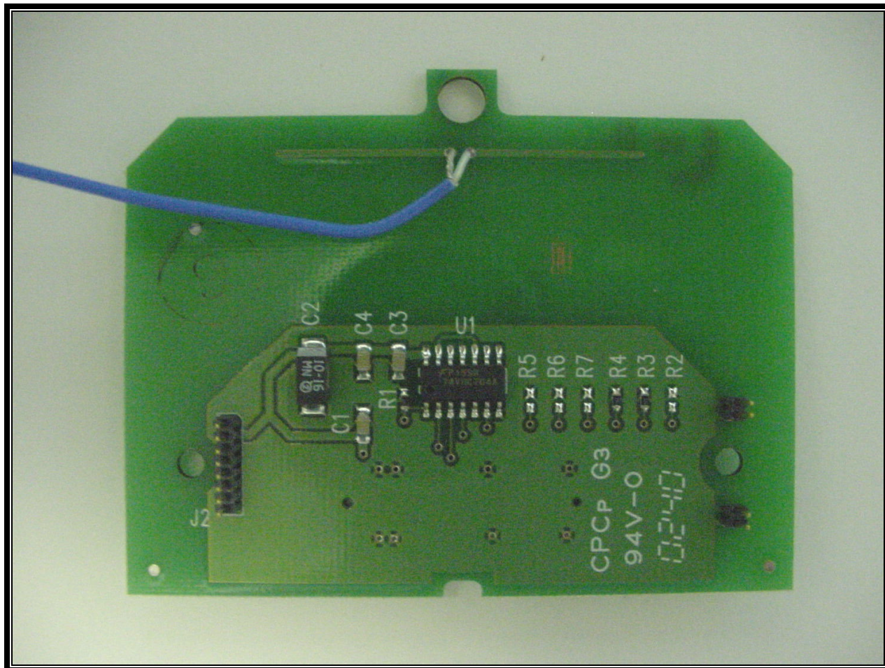
PHOTOGRAPH 39: QL FAMILY (CC16203-2) ANTENNA FRONT VIEW
