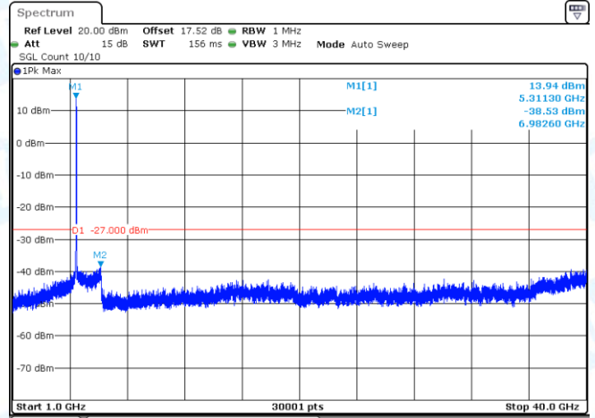
11AC40-CDD-Ant2-5310-1000~40000-PASS
