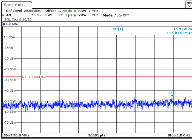
11AC20-CDD-Ant1-5240-30~1000-PASS
