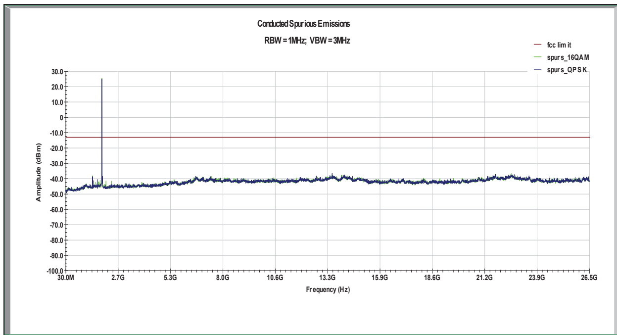
Band 2 Low QPSK and 16-QAM
