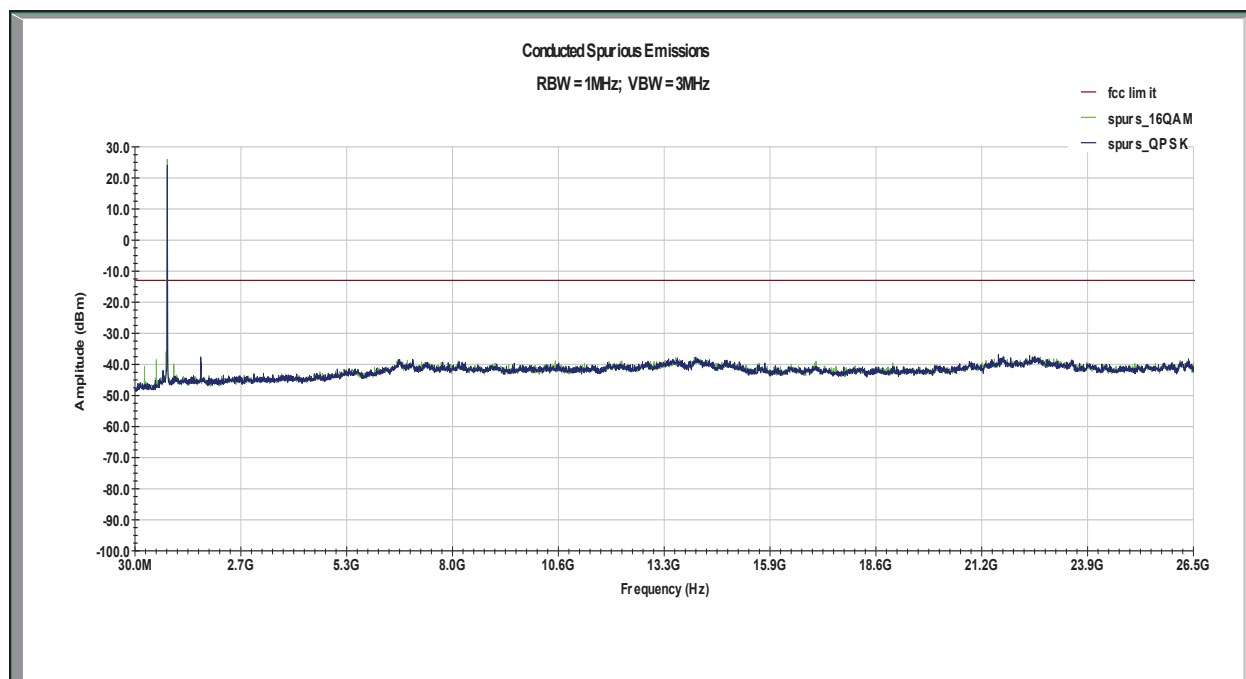
Band 5 Mid QPSK and 16-QAM
