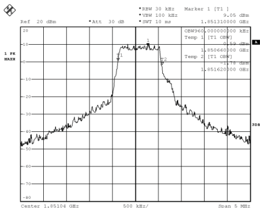
16QAM Band 2 Low Channel (99% bandwidth, 26dB Bandwidth)
