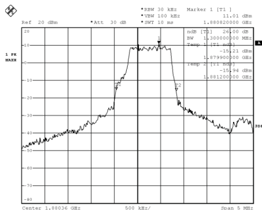
16QAM Band 2 Mid Channel (99% bandwidth, 26dB Bandwidth)
