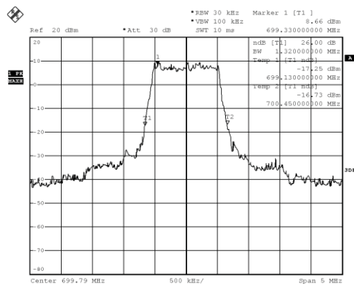
QPSK Band 12 Low Channel (99% bandwidth, 26dB Bandwidth)
