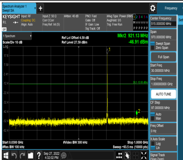
Band12-1.4MHz-16QAM-23173-1RB#0-Range1:30
