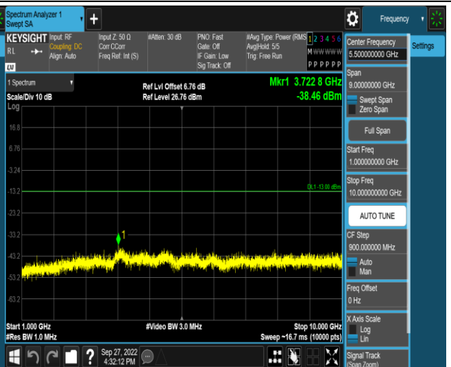
Band12-1.4MHz-16QAM-23173-1RB#0-Range2:1000
