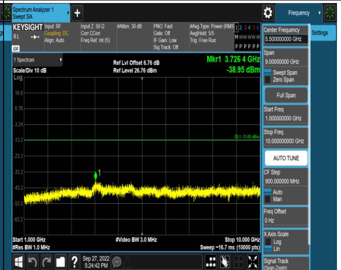
Band17-10MHz-QPSK-23790-1RB#0-Range2:1000~10000MHz
