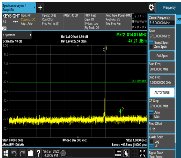
Band12-1.4MHz-QPSK-23095-1RB#0-Range1:30~1000MHz
