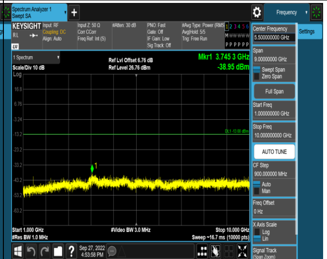
Band12-10MHz-QPSK-23095-1RB#0-Range2:1000~10000MHz
