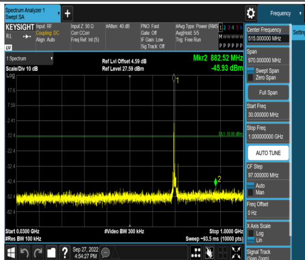
Band12-10MHz-QPSK-23095-1RB#0-Range1:30~1000MHz
