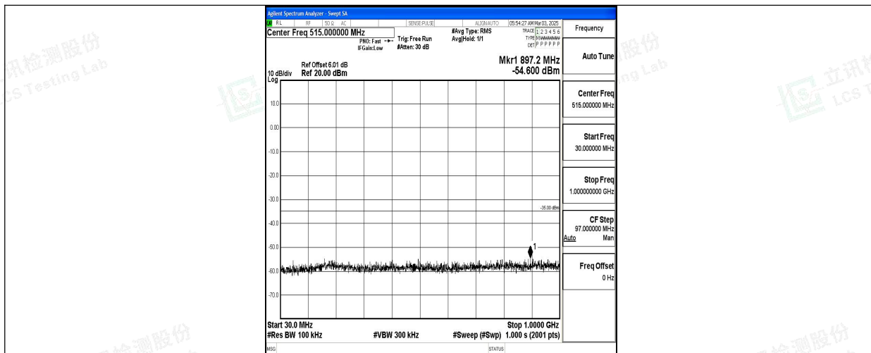
Band7_5MHz_16QAM_21425_1RB#0_30~1000_30~1000
