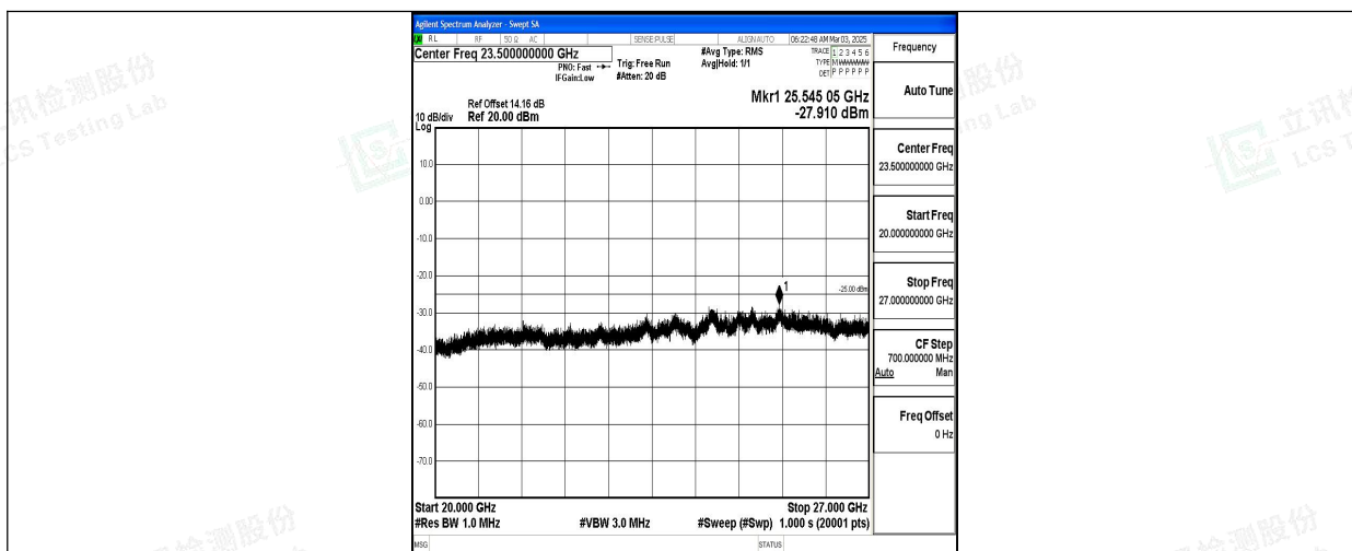
Band7_10MHz_16QAM_20800_1RB#0_20000~27000_20000~27000
