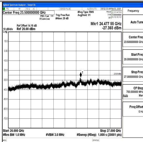
Band7_5MHz_QPSK_21100_1RB#0_20000~27000_20000~27000
