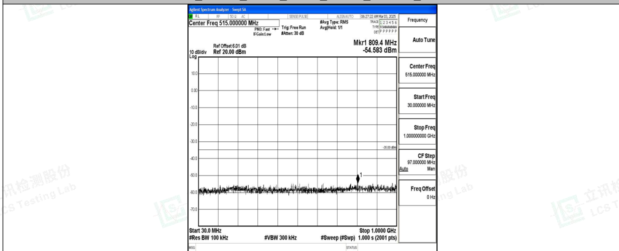
Band7_10MHz_QPSK_21400_1RB#0_30~1000_30~1000
