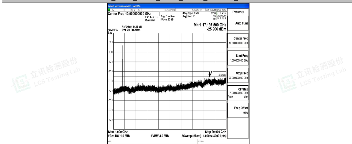
Band7_5MHz_QPSK_21425_1RB#0_1000~20000_1000~20000
