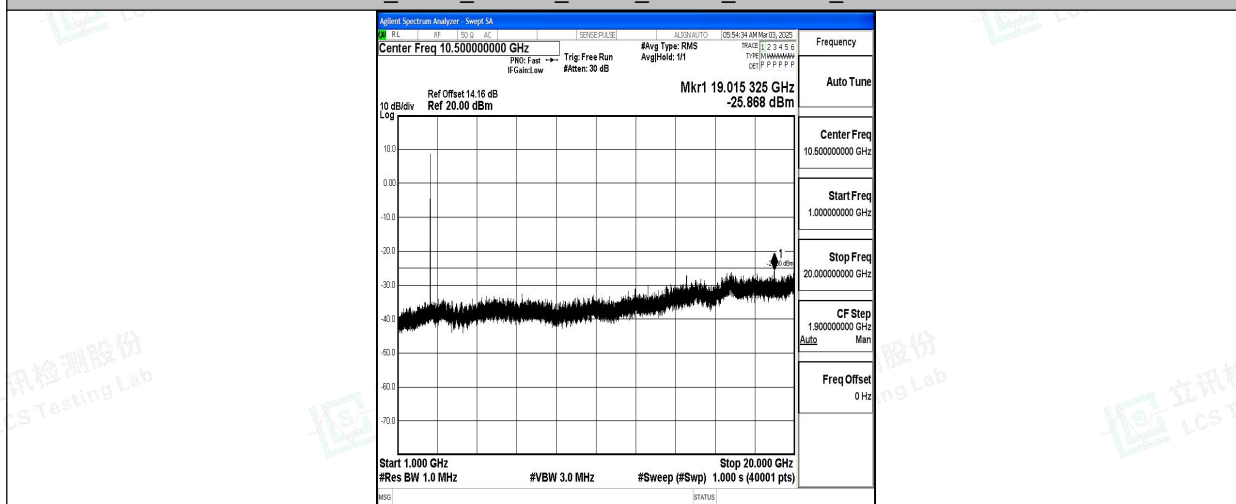
Band7_5MHz_16QAM_21425_1RB#0_1000~20000_1000~20000
