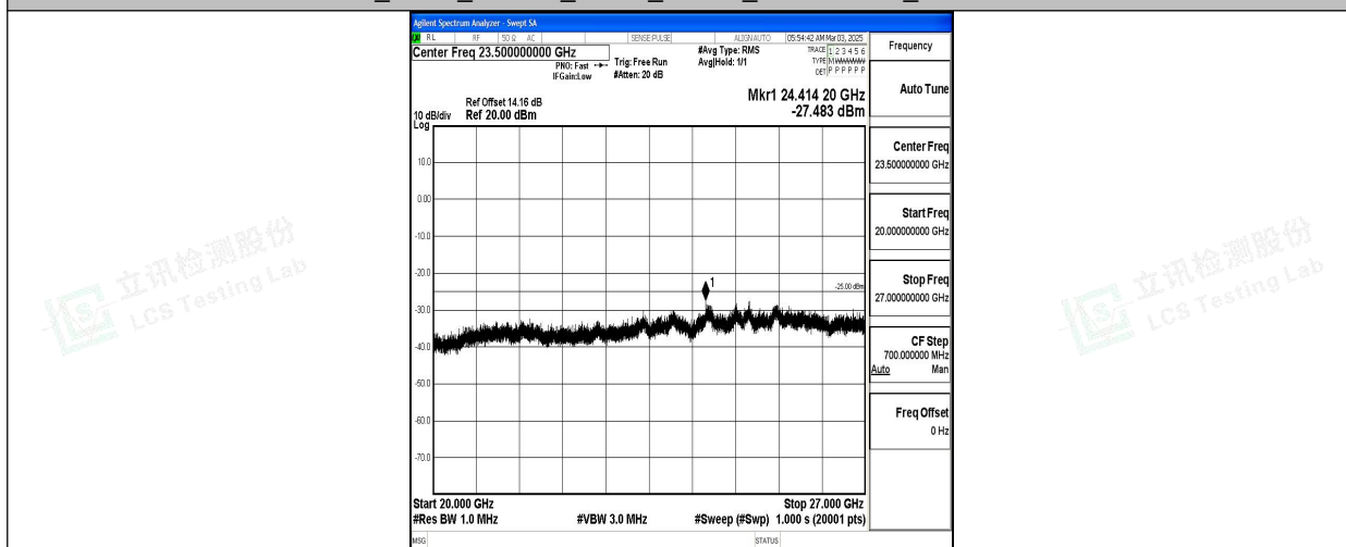
Band7_5MHz_16QAM_21425_1RB#0_20000~27000_20000~27000
