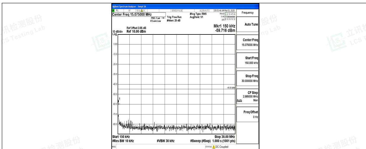
Band7_5MHz_QPSK_21425_1RB#0_0.15~30_0.15~30
