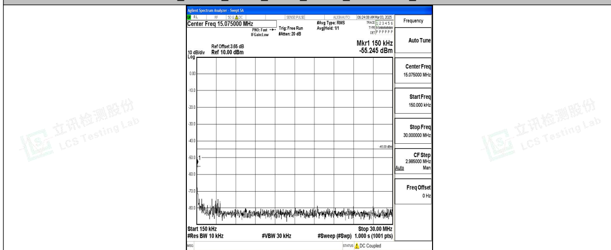
Band7_10MHz_QPSK_21100_1RB#0_0.15~30_0.15~30
