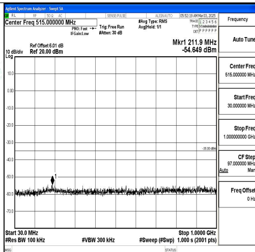
Band7_5MHz_QPSK_21100_1RB#0_30~1000_30~1000
