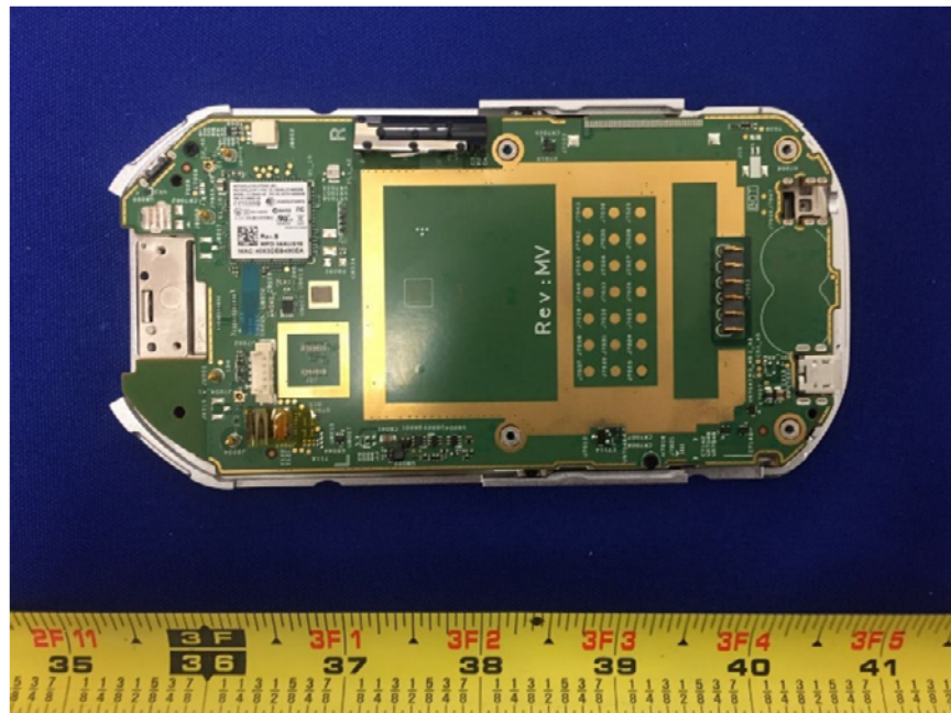
UZ7211486030B Radio Board View
