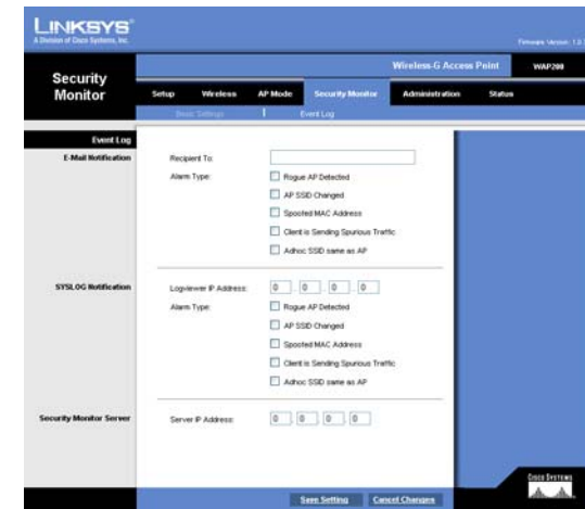
Figure 6-21: Security Monitor - Event Log
