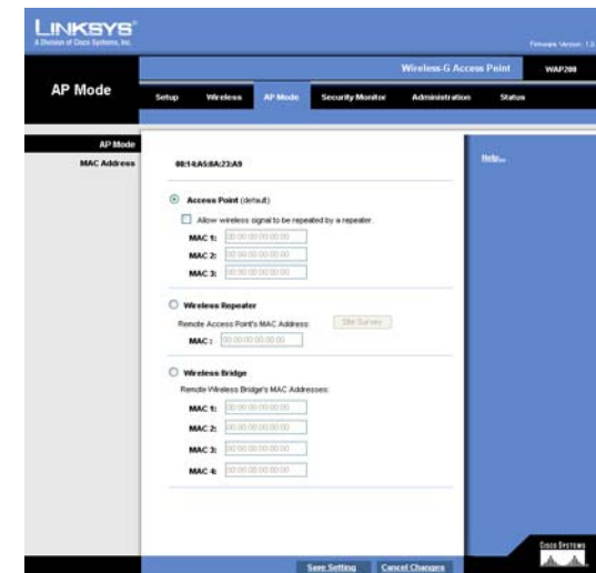
Figure 6-17: AP Mode
