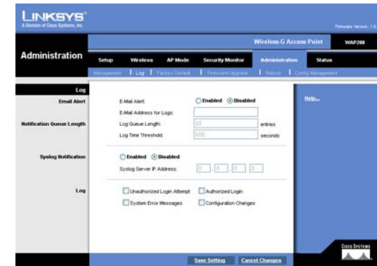
Figure 6-23: Administration - Log
