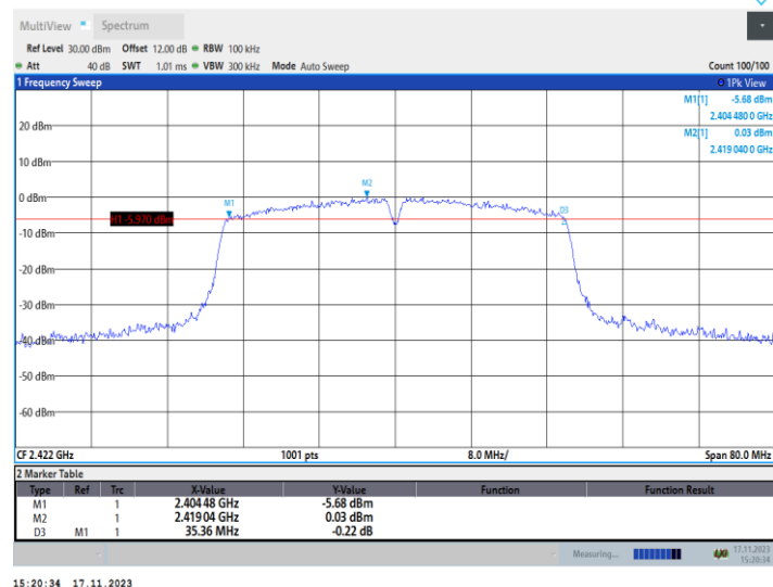
11AC40MIMO Ant2 2422
