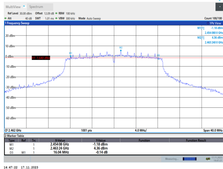
11AC20MIMO Ant2 2462
