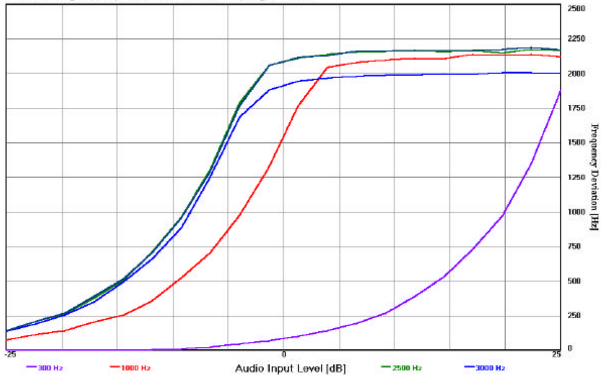
RTL Modulation Limiting Response (154.57 MHz : 12.5 kHz Channel Spacing) Positive Peak
