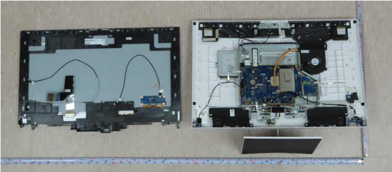
Open View of EUT
