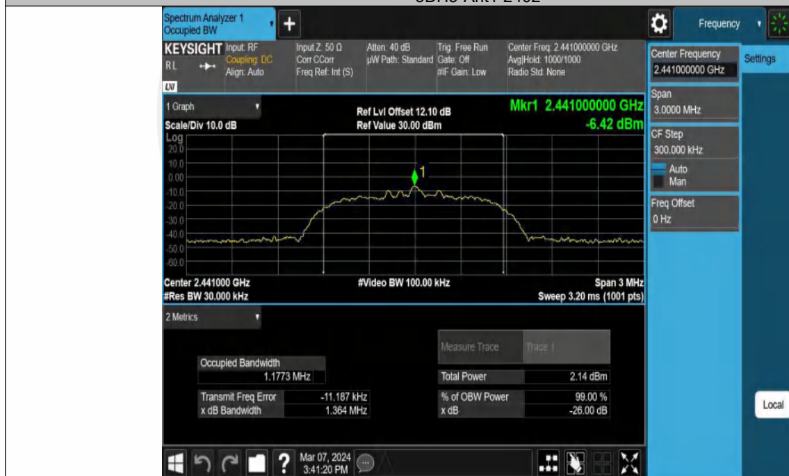
3DH5-Ant1-2441
