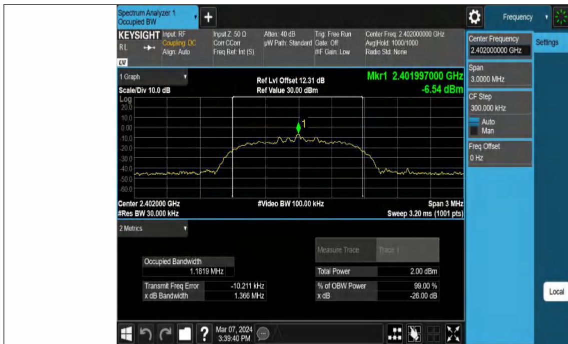
3DH5-Ant1-2402
