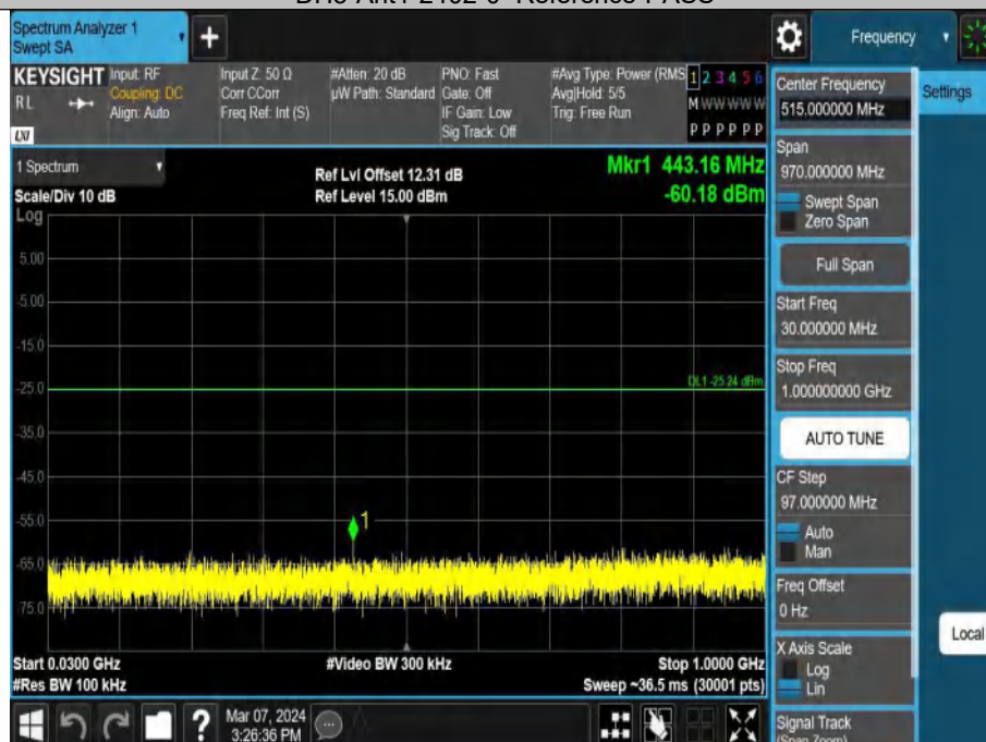
DH5-Ant1-2402-30~1000-PASS
