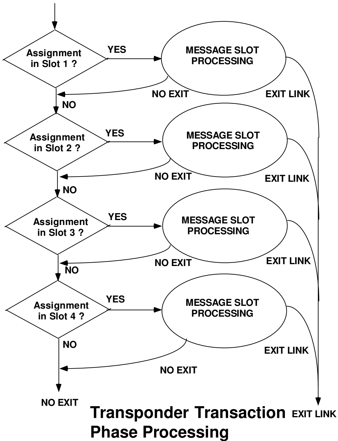
Figure 5-3c: Transaction Phase Processing
