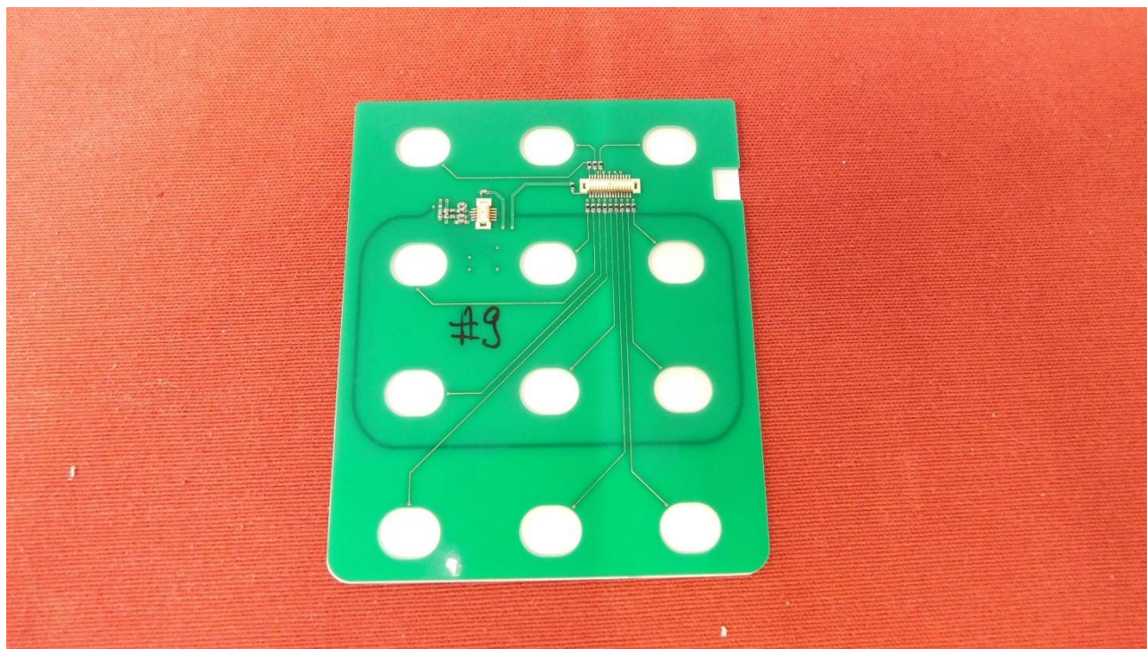
Picture 5: Touch PCB – bottom side
