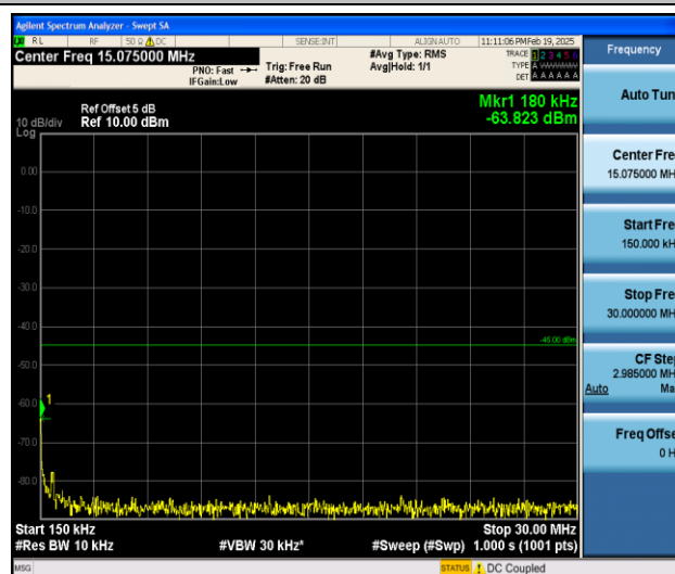
Band7_20MHz_16QAM_21350_1RB#0_0.15~30_0.15~30
