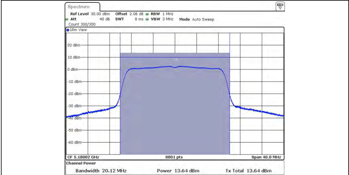
11AC20SISO_Ant1_5180
