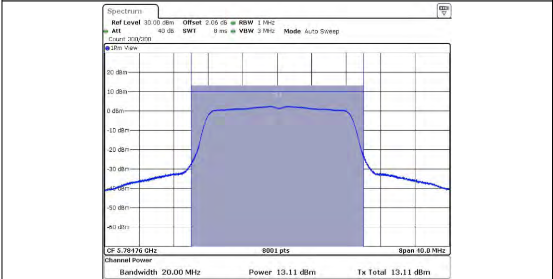
11A_Ant1_5785
