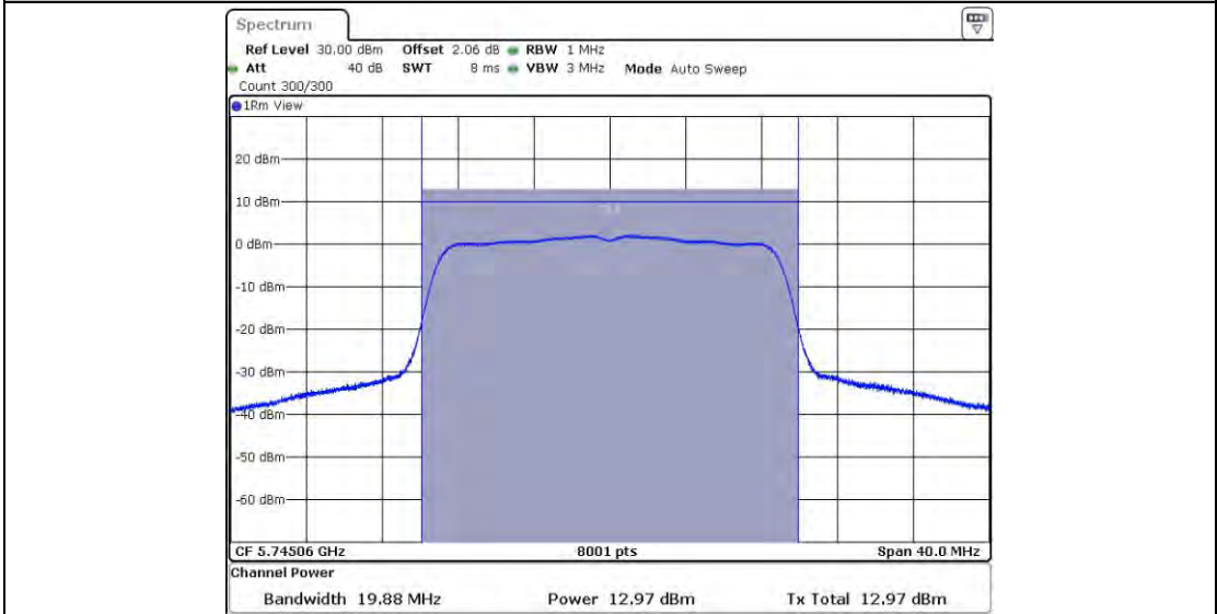
11AC20SISO_Ant1_5745
