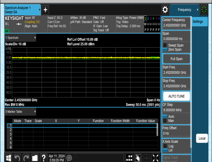
NTNV-11N40MIMO-Ant2-2452
