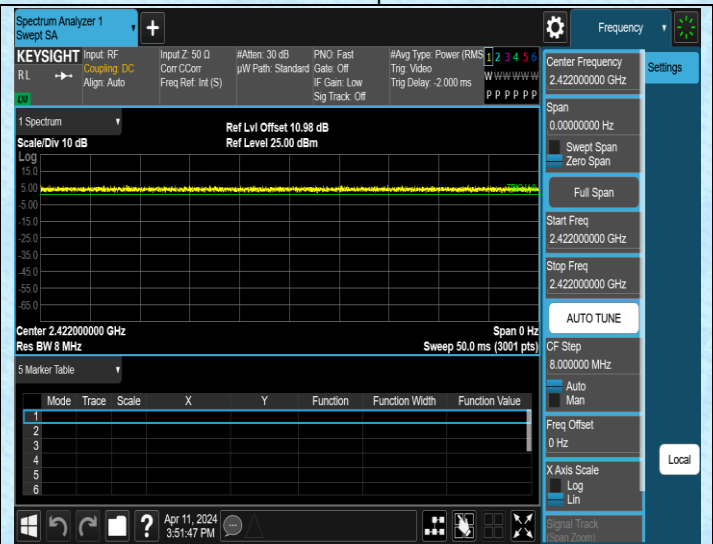
NTNV-11N40MIMO-Ant2-2422
