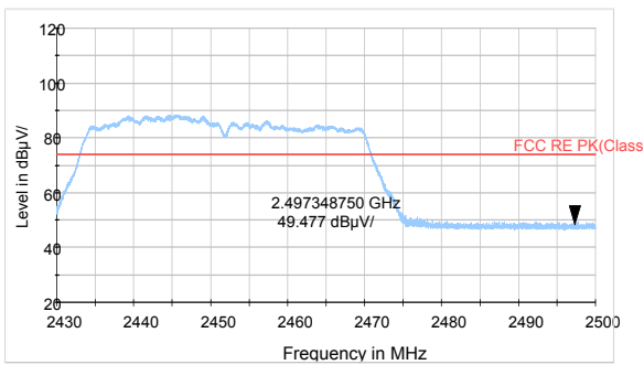
802.11n HT40 -Channel 9 Peak
