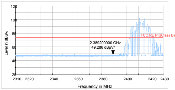
802.11b-Channel 1 Peak
