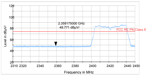
802.11n HT40 -Channel 3 Peak
