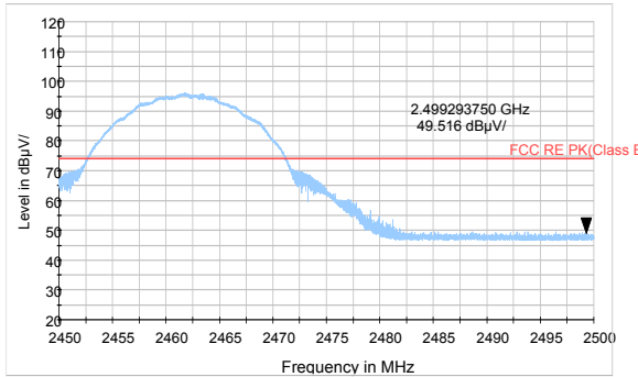
802.11b-Channel 11 Peak
