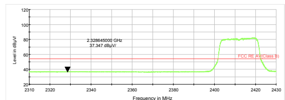
802.11n HT20 -Channel 1 Average
