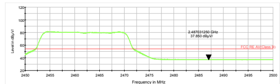
802.11g-Channel 11 Average
