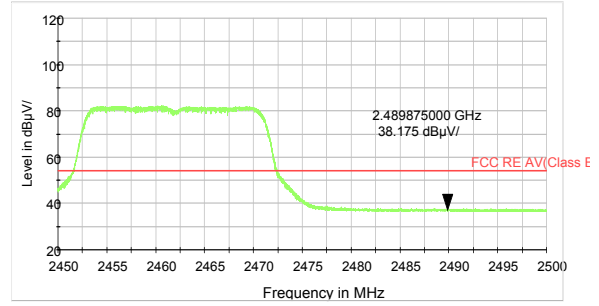
802.11n HT20 -Channel 11 Average
