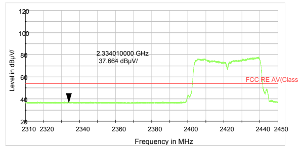
802.11n HT40 -Channel 3 Average
