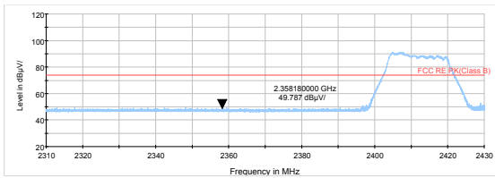
802.11g-Channel 1 Peak
