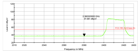
802.11g-Channel 1 Average
