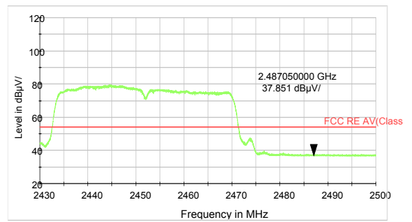
802.11n HT40 -Channel 9 Average
