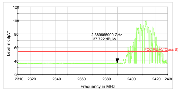
802.11b-Channel 1 Average
