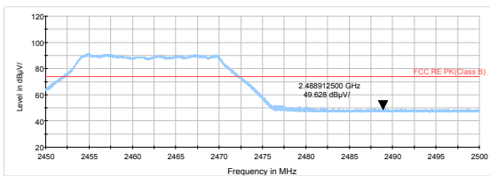
802.11g-Channel 11 Peak
