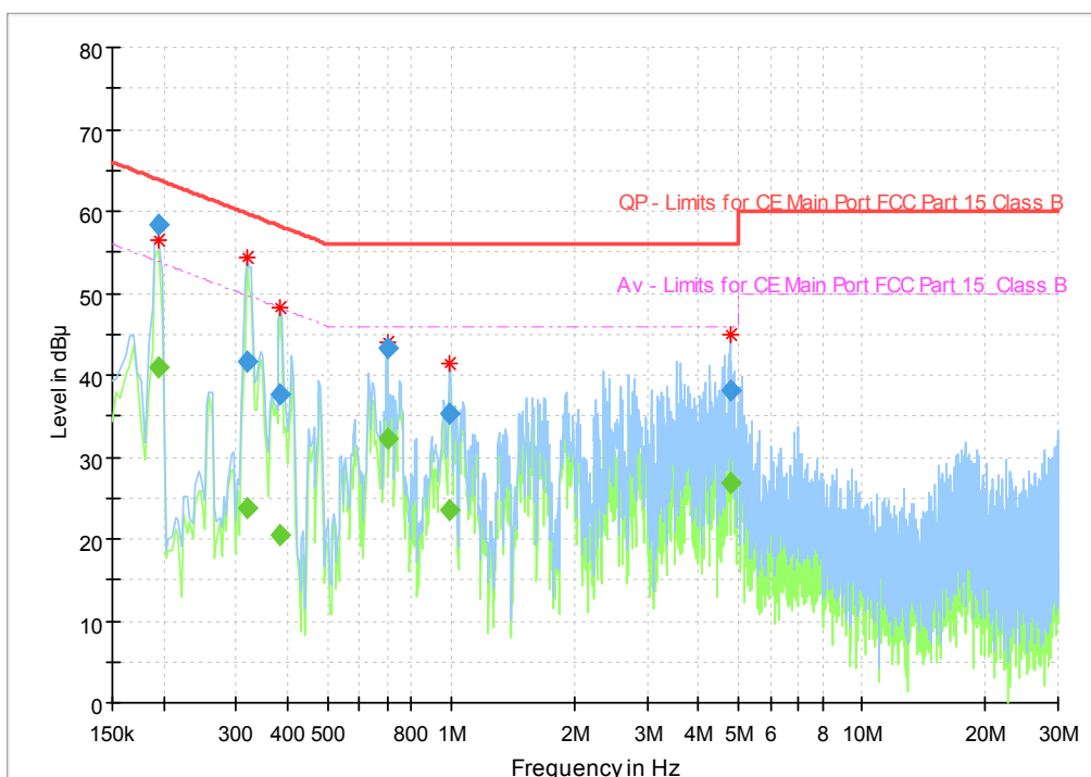
Fig. 58 Conducted Emission(802.11a, TX)
