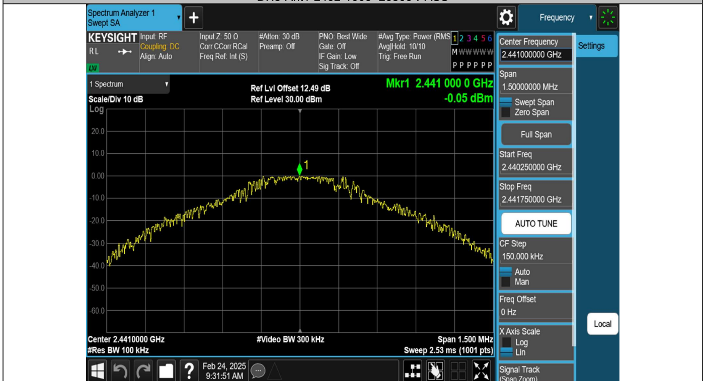
DH5-Ant1-2441-0~Reference-PASS
