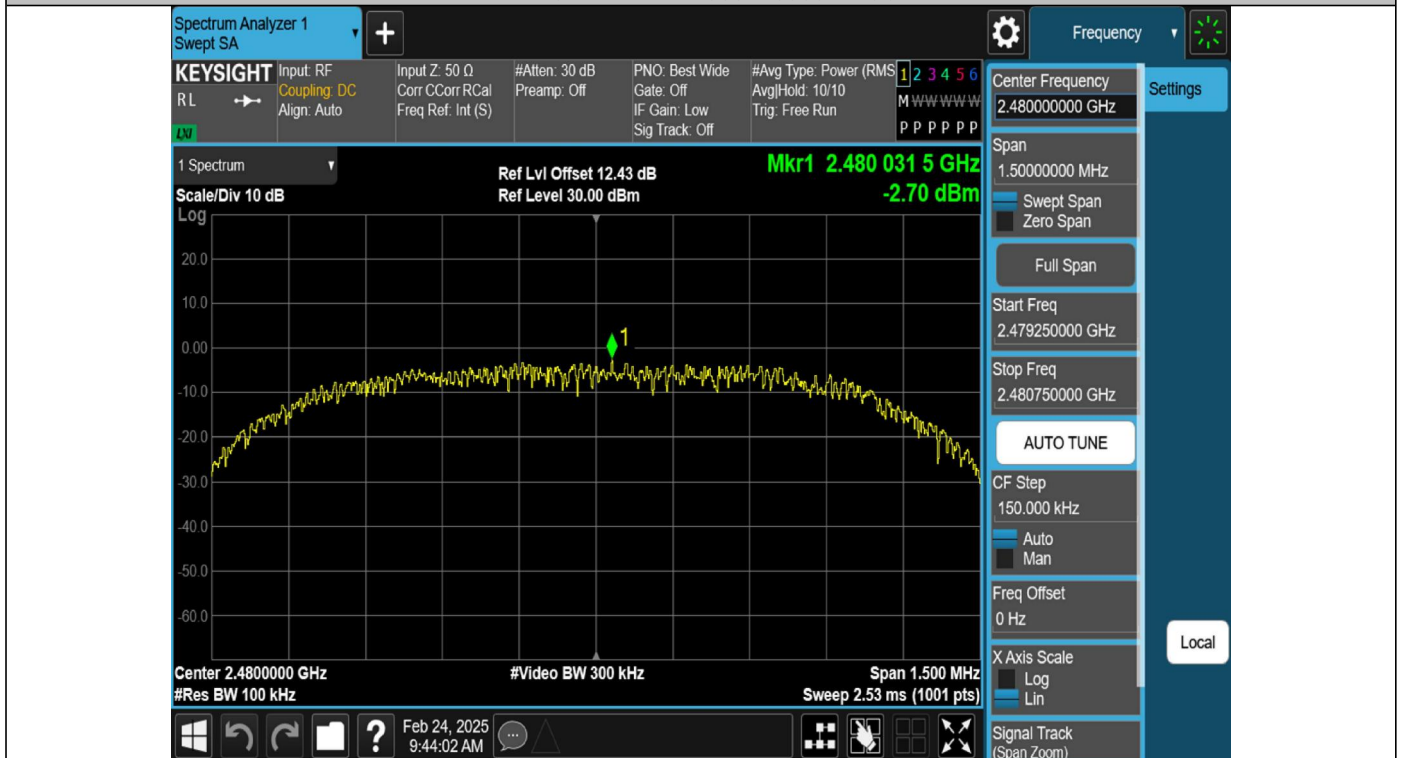
2DH5-Ant1-2480-0~Reference-PASS
