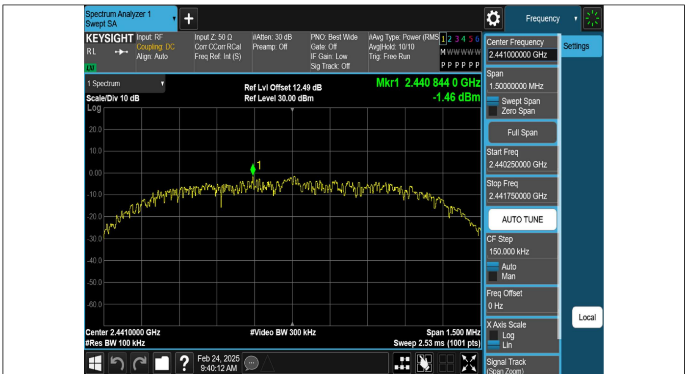
2DH5-Ant1-2441-0~Reference-PASS
