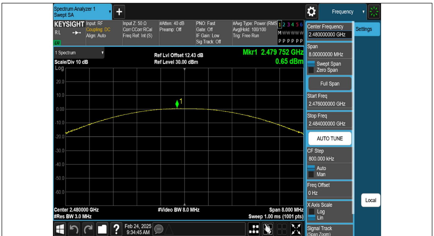
DH5-Ant1-2480-PASS
