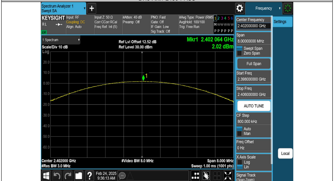
2DH5-Ant1-2402-PASS
