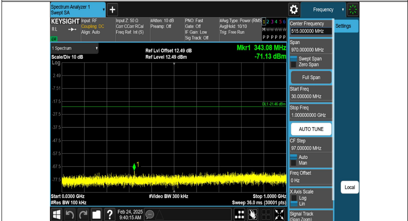
2DH5-Ant1-2441-30~1000-PASS
