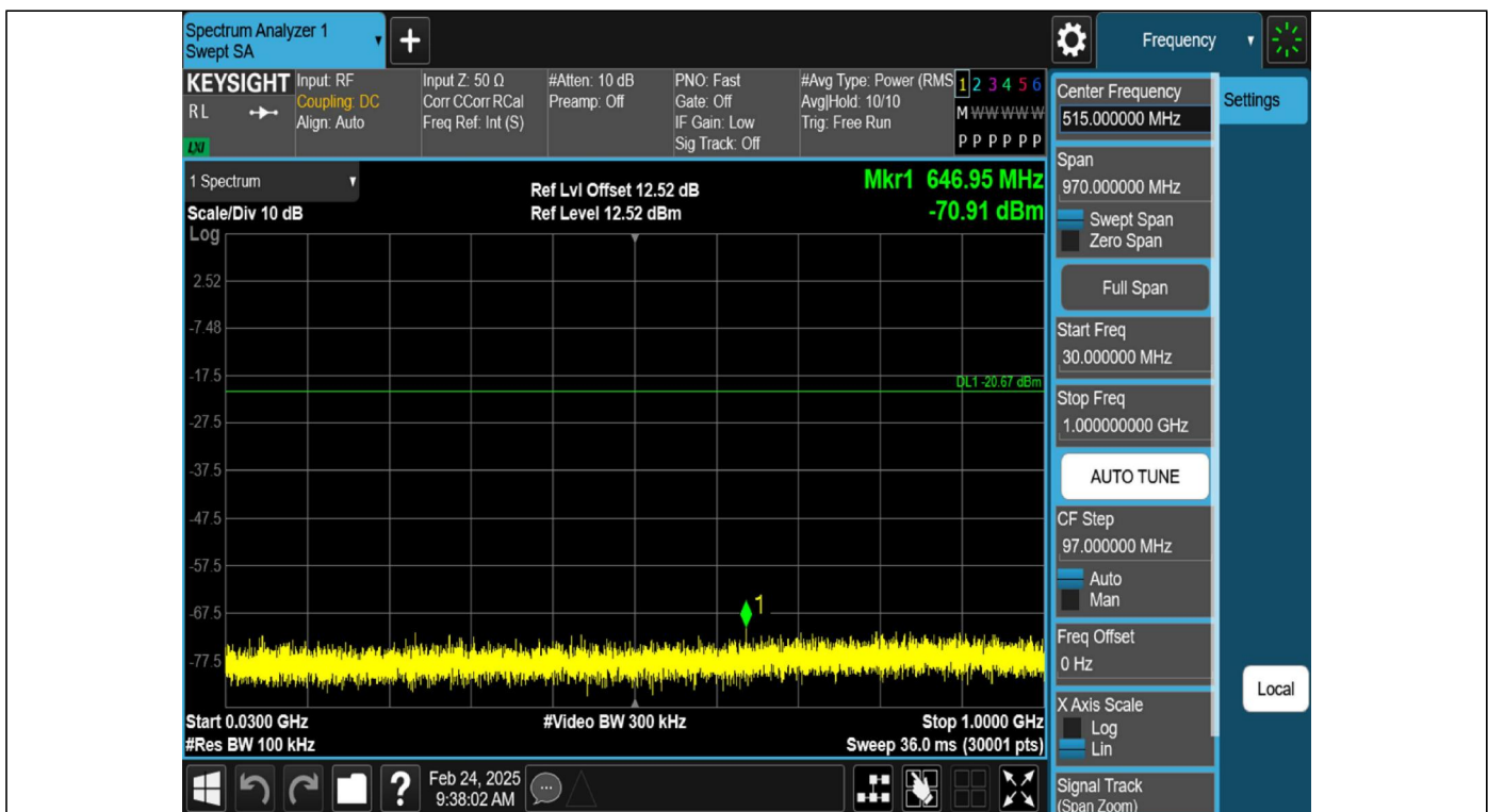
2DH5-Ant1-2402-30~1000-PASS
