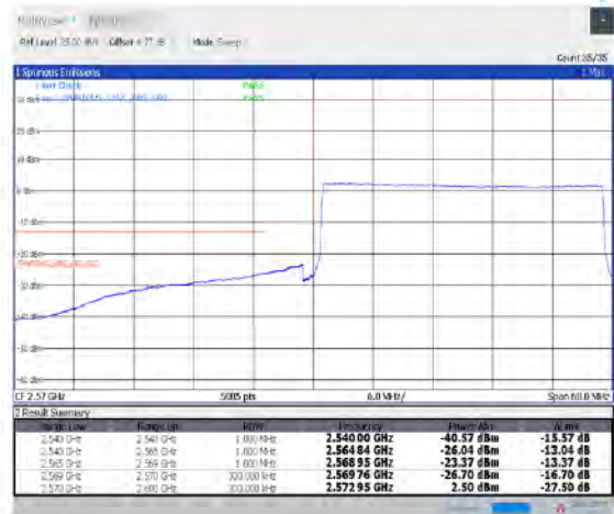
1-N38--30-30-L-6-CP-QPSK-Outer_Full-78@0-Ant1-PASS-see graph
