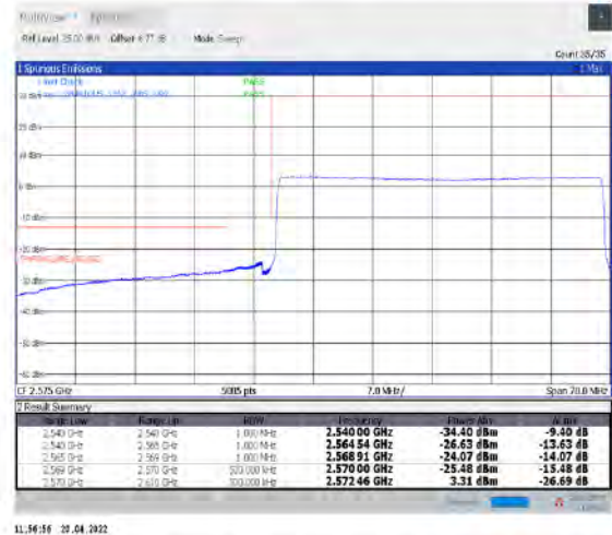
1-N38--30-40-L-6-CP-QPSK-Outer_Full-106@0-Ant1-PASS-see graph
