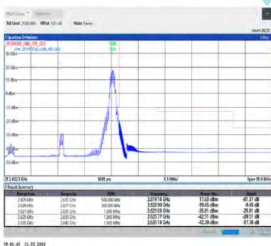
1-N38-PC2-30-15-H-5-CP-QPSK-Edge_1RB_Right-1@37-Ant1-PASS-see graph
