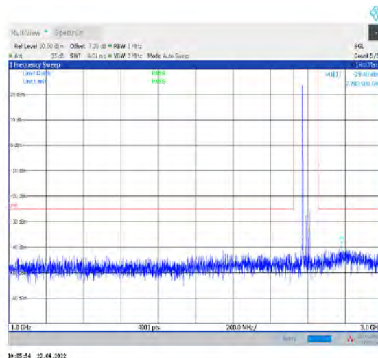
1-N38--30-40-L-1-DFT-PI2BPSK-Inner_1RB_Left- 1@1-1000-3000-Ant1--39.40--25-PASS
