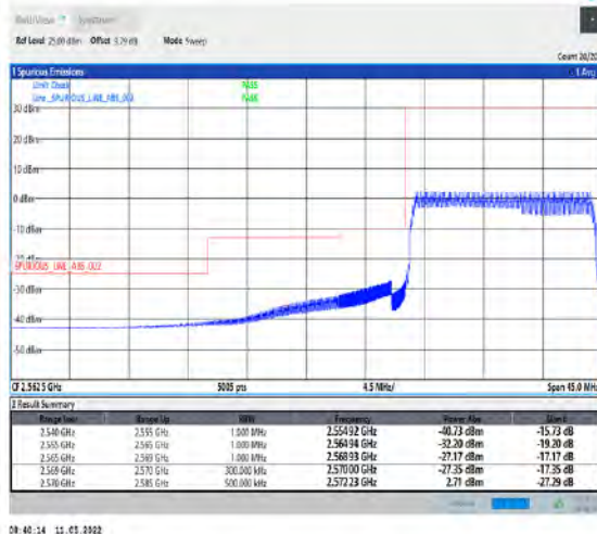
1-N38-PC2-30-15-L-6-CP-QPSK-Outer_Full-38@0-Ant1-PASS-see graph
