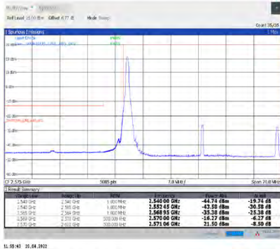
1-N38--30-40-L-4-CP-QPSK-Edge_1RB_Left-1@0-Ant1-PASS-see graph
