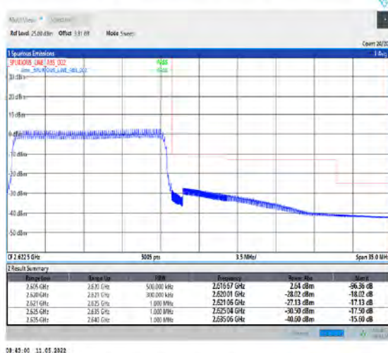
1-N38-PC2-30-15-H-6-CP-QPSK-Outer_Full-38@0-Ant1-PASS-see graph
