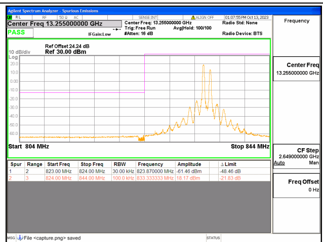
5B / 10+10MHz / Low CH / QPSK / 1#49-1#0
