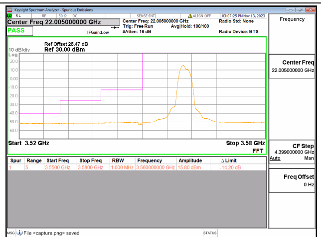
48C / 10+20MHz / Low CH / QPSK / 1#49-1#0
