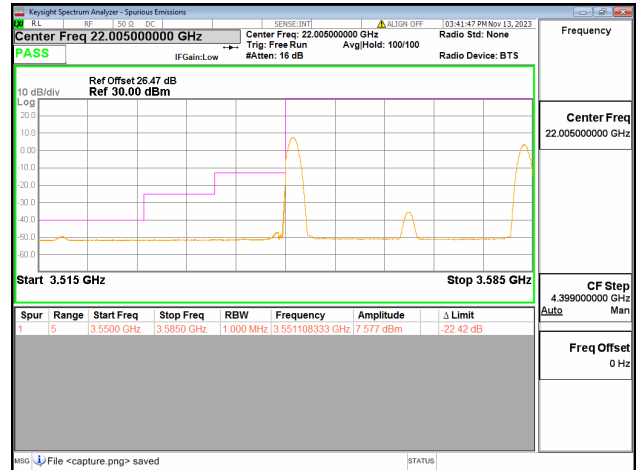
48C / 20+15MHz / Low CH / QPSK / 1#0-1#74
