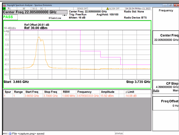
48C / 15+20MHz / High CH / QPSK / 1#74-1#0
