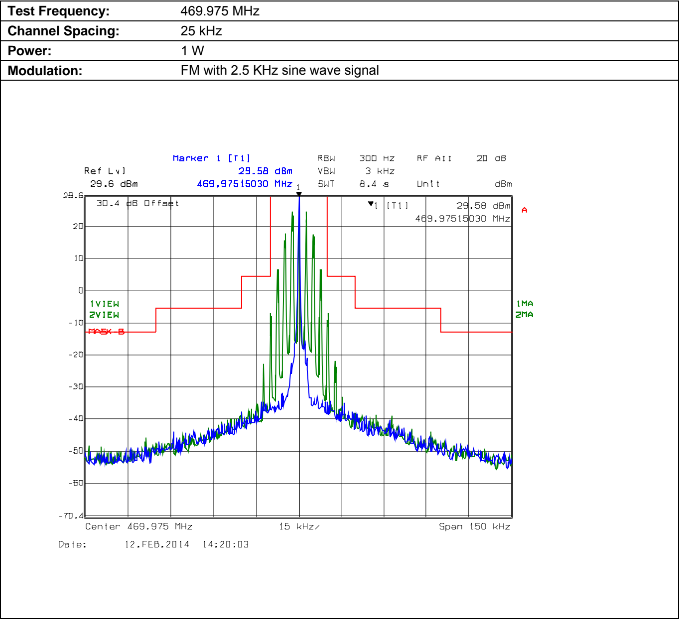
Plot 5.8.4.3.3. Emission Mask B, High Power
