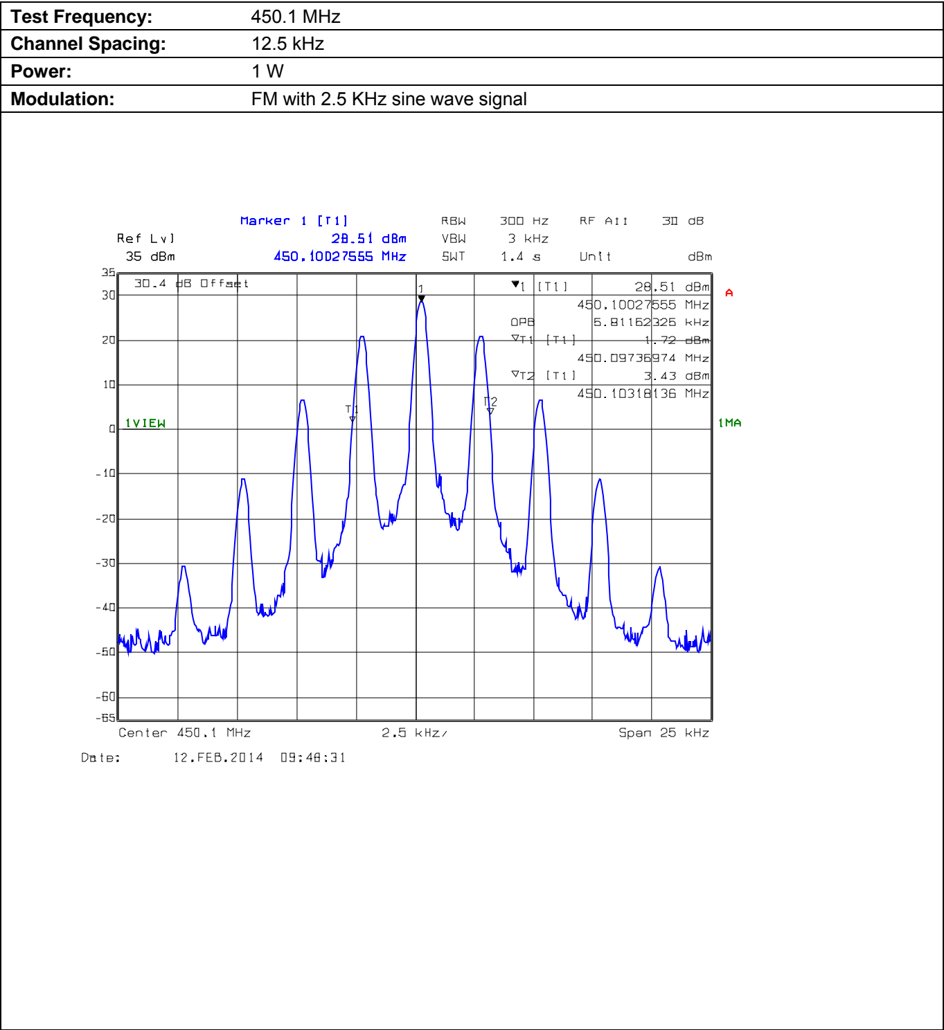
Plot 5.8.4.1.2. Occupied Bandwidth
