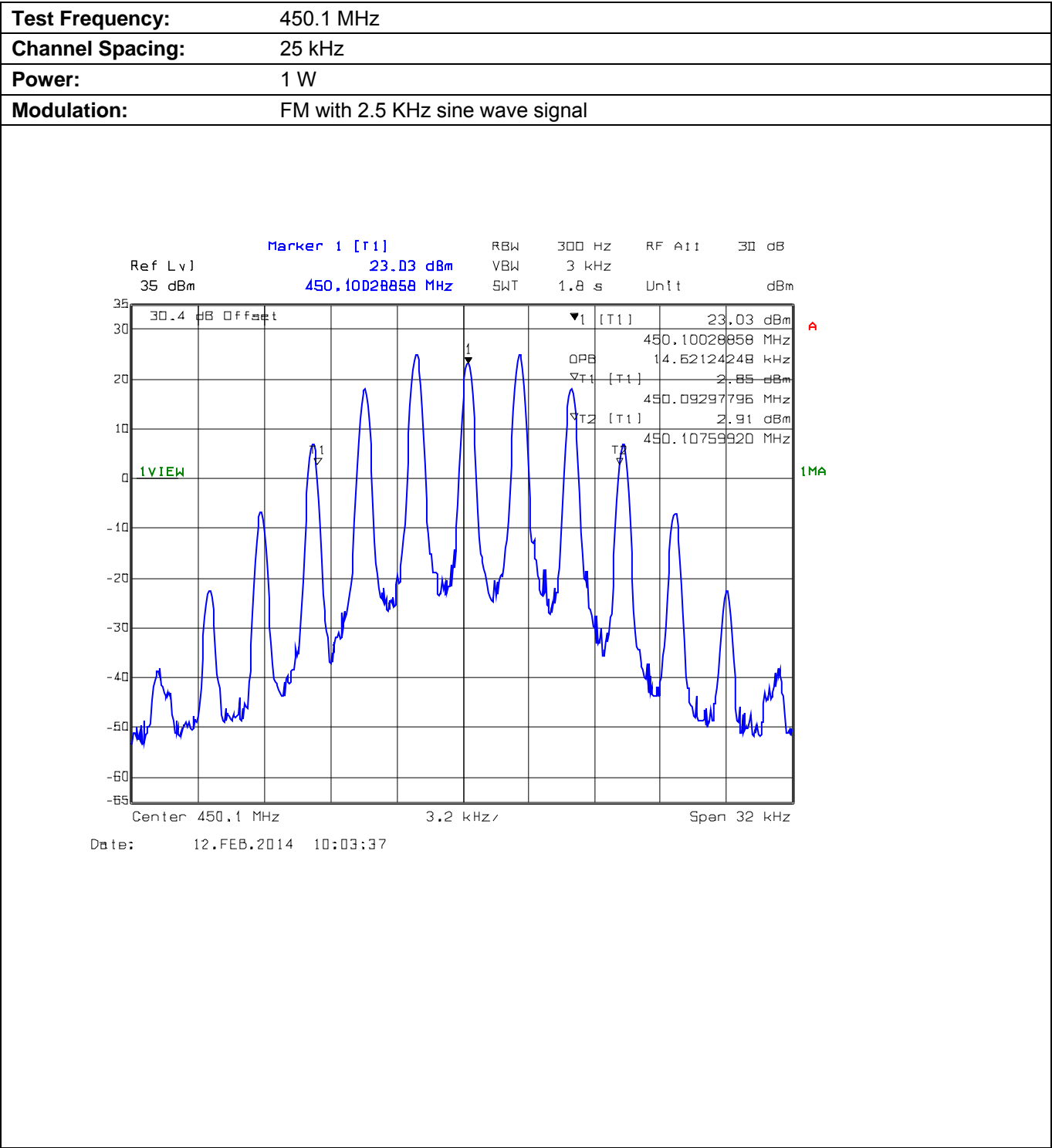
Plot 5.8.4.1.5. Occupied Bandwidth
