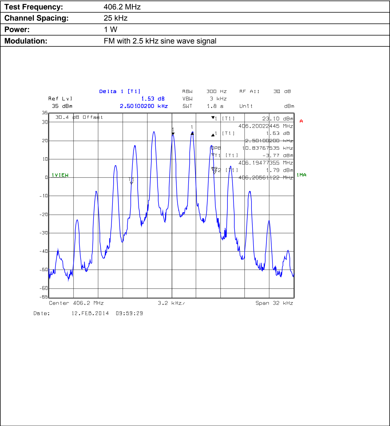
Plot 5.8.4.1.4. Occupied Bandwidth
