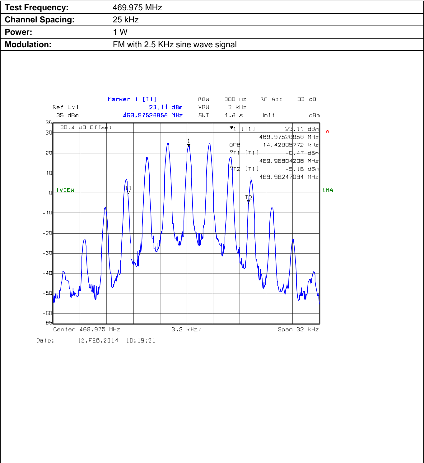
Plot 5.8.4.1.6. Occupied Bandwidth
