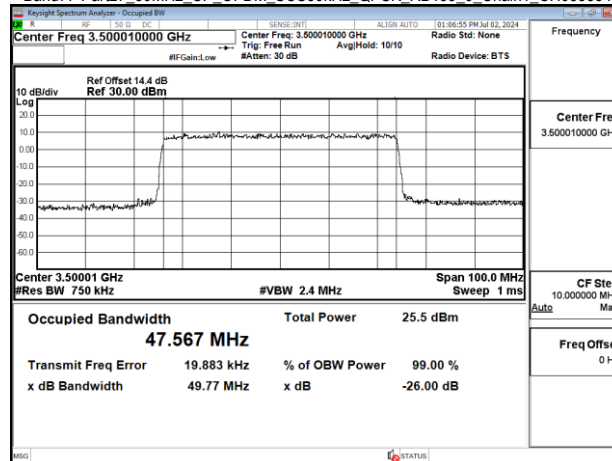
Band77-Part27_50MHz_CP_OFDM_SCS30kHz_QPSK_RB133_0_Chain1_CH633334
