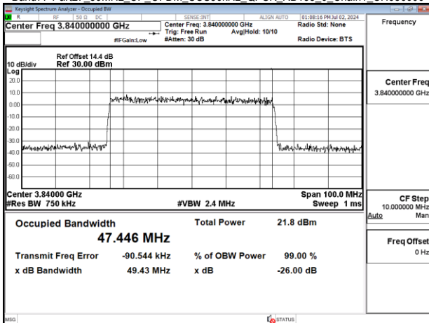
Band77-Part27_50MHz_CP_OFDM_SCS30kHz_QPSK_RB133_0_Chain1_CH656000
