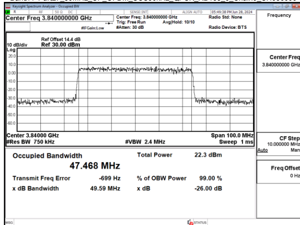
Band77-Part27_50MHz_CP_OFDM_SCS30kHz_QPSK_RB133_0_Chain0_CH656000
