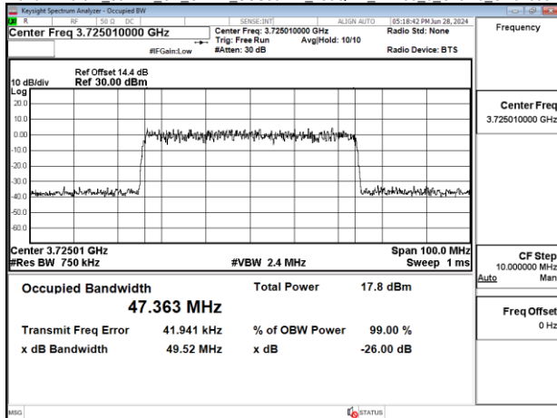
Band77-Part27_50MHz_CP_OFDM_SCS30kHz_256QAM_RB133_0_Chain0_CH656000
