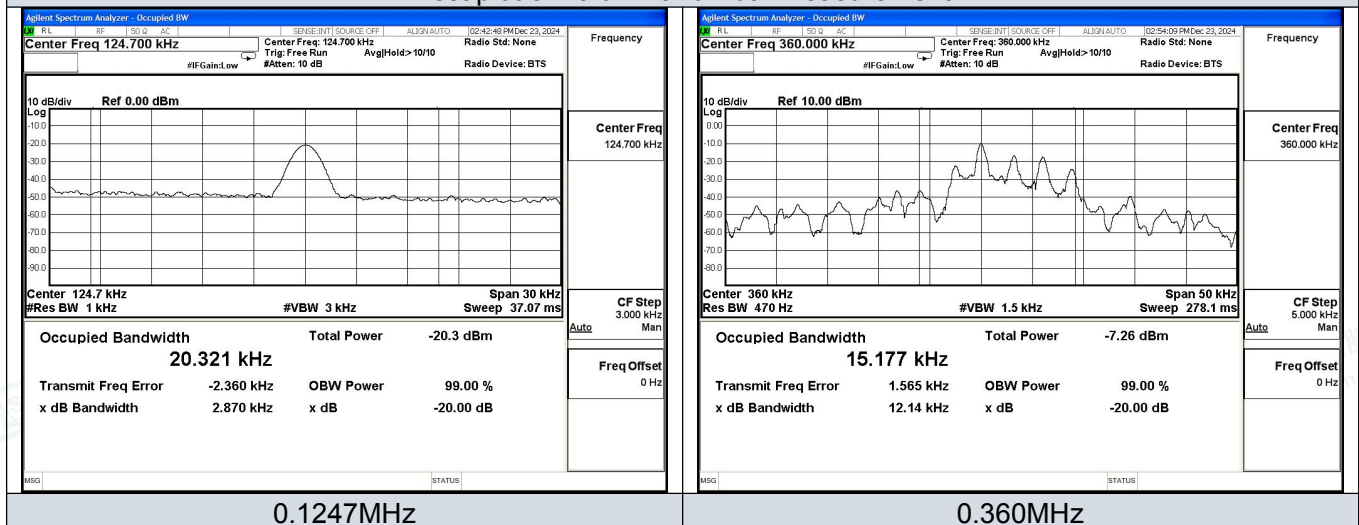
Test plot of 20 dB Bandwidth Measurement
