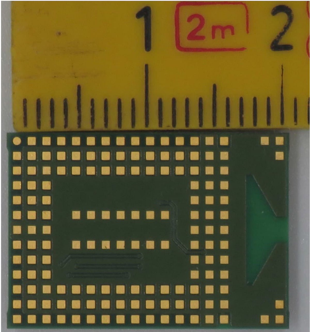
IRIS-W106-00B – bottom view
