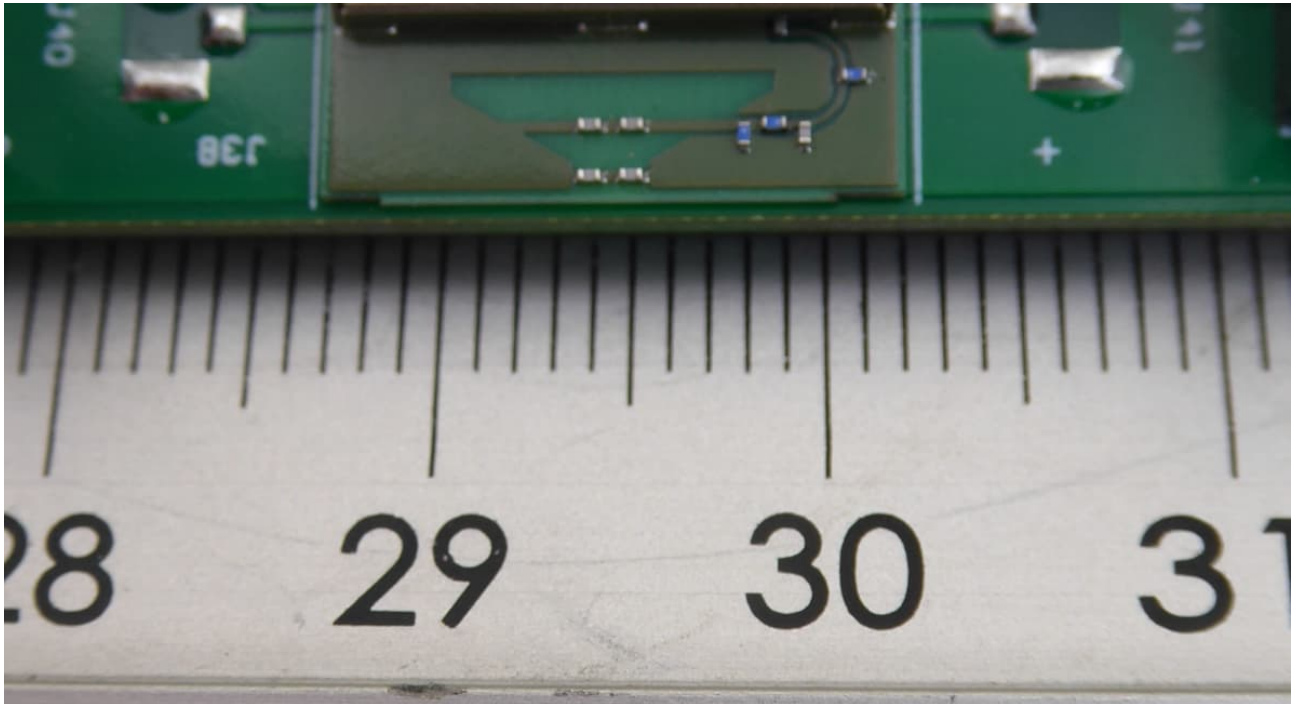
Abracon PCB trace antenna (On-board antenna on the IRIS-W106-00B)
