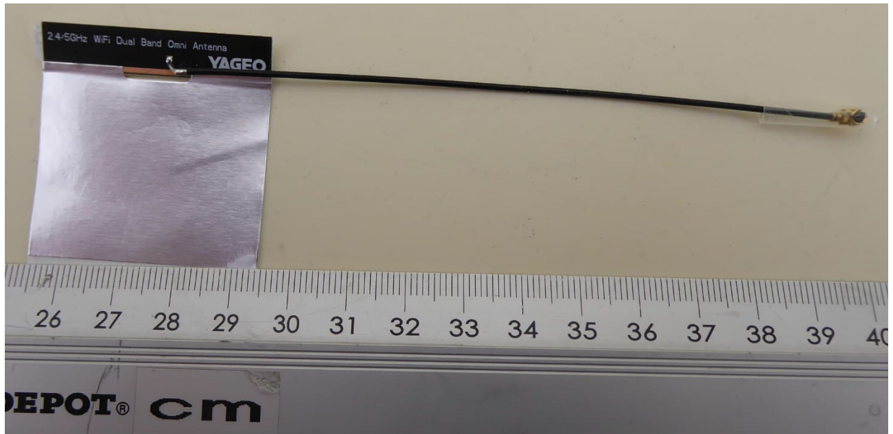
PCB Patch antenna ANTX100P002B24553 by Pulse Electronics / Yageo
