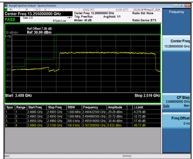
Band41_20MHz_QPSK_39750_100RB#0
