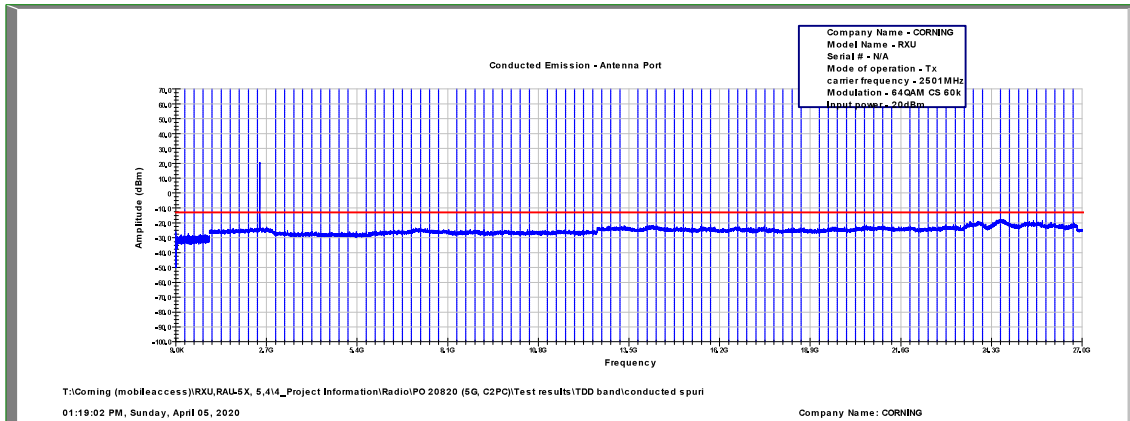
Figure 501: Spurious Emissions at Antenna Terminal 64QAM, 2501.0MHz, B.W. 10MHz, Sub Carrier 60kHz
