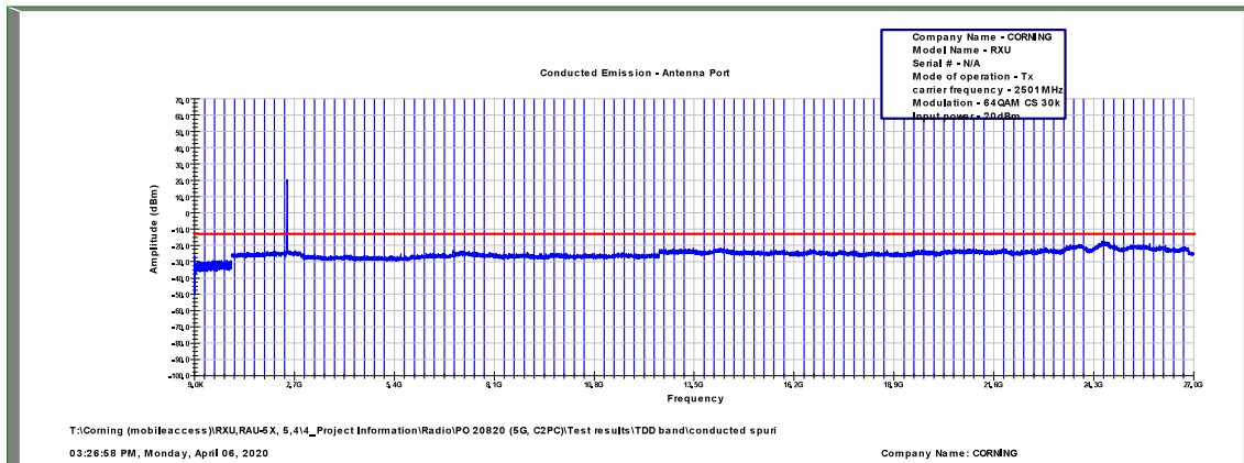
Figure 498: Spurious Emissions at Antenna Terminal 64QAM, 2501.0MHz, B.W. 10MHz, Sub Carrier 30kHz
