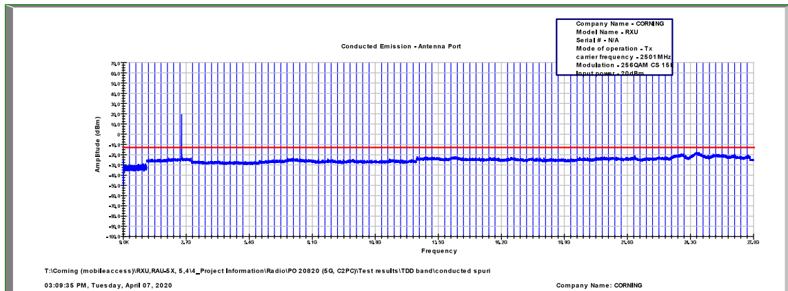
Figure 543: Spurious Emissions at Antenna Terminal 256QAM, 2501.0MHz, B.W. 10MHz, Sub Carrier 15kHz
