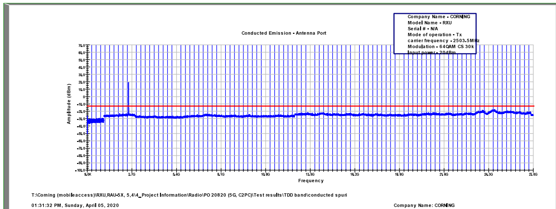
Figure 507: Spurious Emissions at Antenna Terminal 64QAM, 2503.5MHz, B.W. 15MHz, Sub Carrier 30kHz
