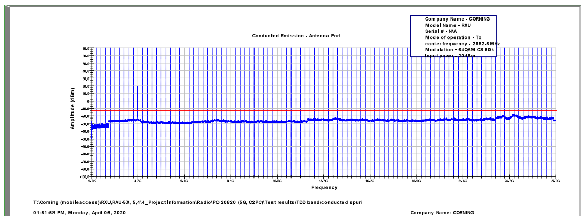
Figure 512: Spurious Emissions at Antenna Terminal 64QAM, 2682.5MHz, B.W. 15MHz, Sub Carrier 60kHz
