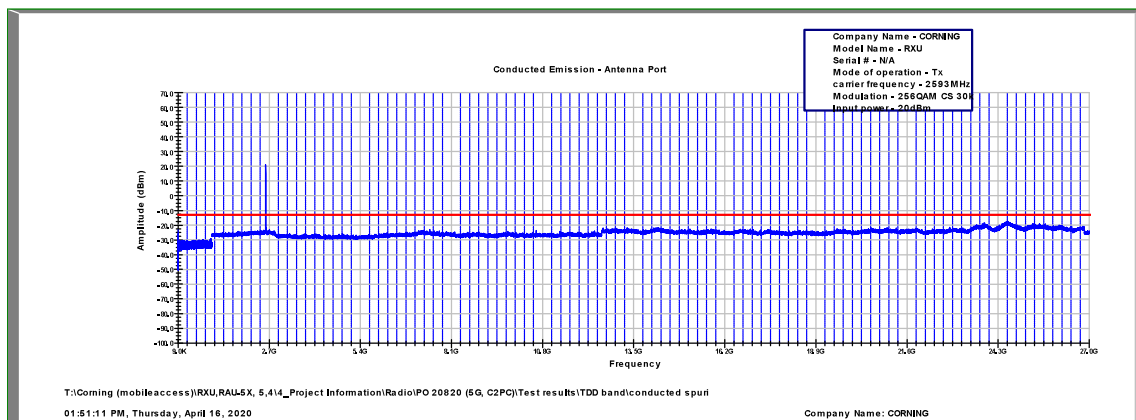
Figure 541: Spurious Emissions at Antenna Terminal 256QAM, 2593.0MHz, B.W. 5MHz, Sub Carrier 30kHz
