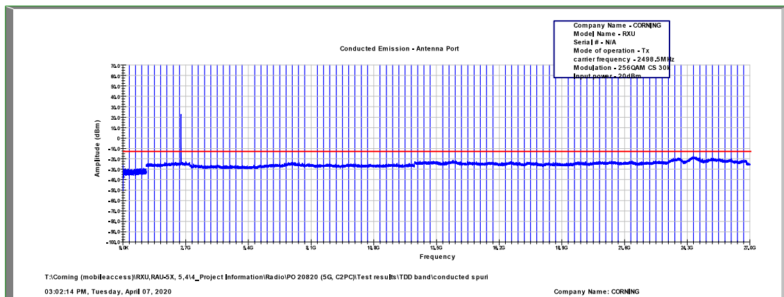
Figure 540: Spurious Emissions at Antenna Terminal 256QAM, 2498.5MHz, B.W. 5MHz, Sub Carrier 30kHz
