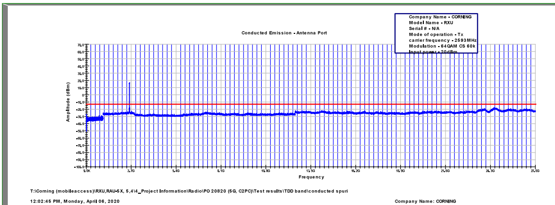
Figure 520: Spurious Emissions at Antenna Terminal 64QAM, 2593.0MHz, B.W. 20MHz, Sub Carrier 60kHz
