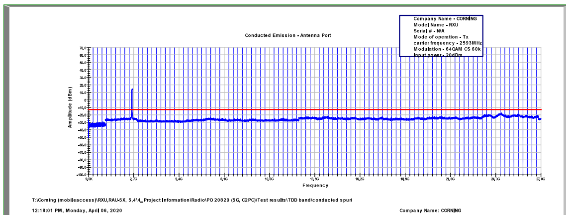
Figure 529: Spurious Emissions at Antenna Terminal 64QAM, 2593.0MHz, B.W. 40MHz, Sub Carrier 60kHz
