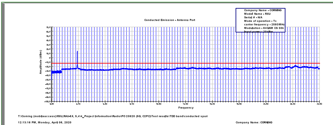
Figure 526: Spurious Emissions at Antenna Terminal 64QAM, 2593.0MHz, B.W. 40MHz, Sub Carrier 30kHz
