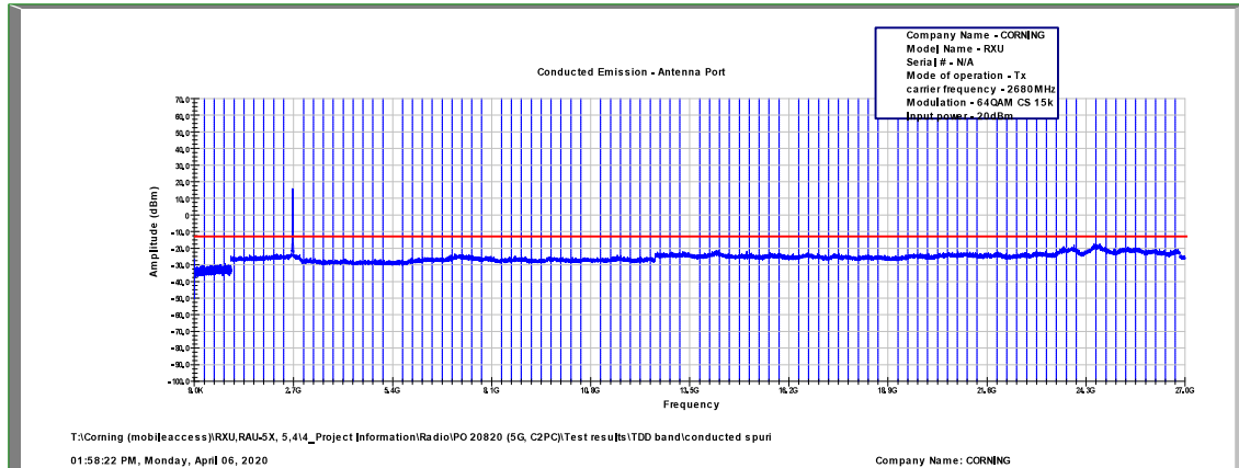
Figure 515: Spurious Emissions at Antenna Terminal 64QAM, 2680.0MHz, B.W. 20MHz, Sub Carrier 15kHz
