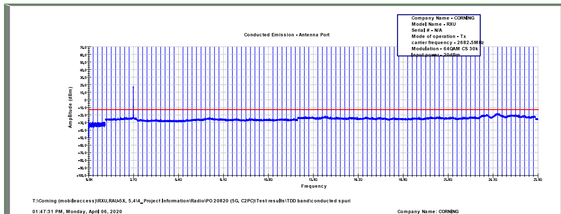
Figure 509: Spurious Emissions at Antenna Terminal 64QAM, 2682.5MHz, B.W. 15MHz, Sub Carrier 30kHz
