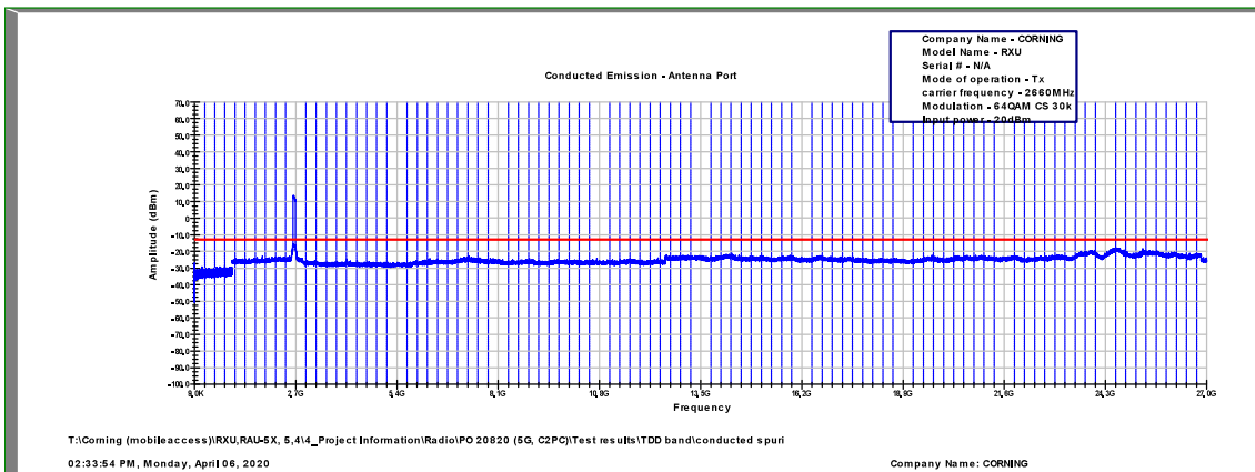
Figure 533: Spurious Emissions at Antenna Terminal 64QAM, 2660.0MHz, B.W. 60MHz, Sub Carrier 30kHz
