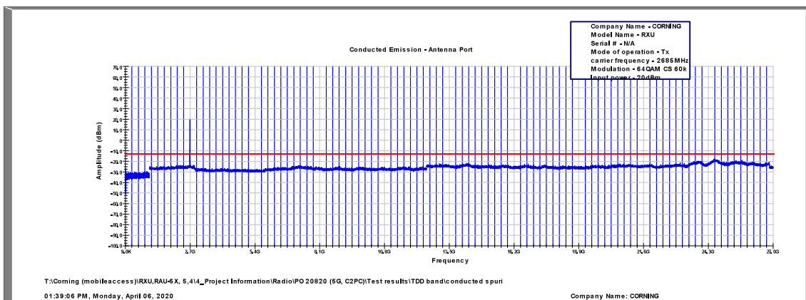
Figure 503: Spurious Emissions at Antenna Terminal 64QAM, 2685.0MHz, B.W. 10MHz, Sub Carrier 60kHz
