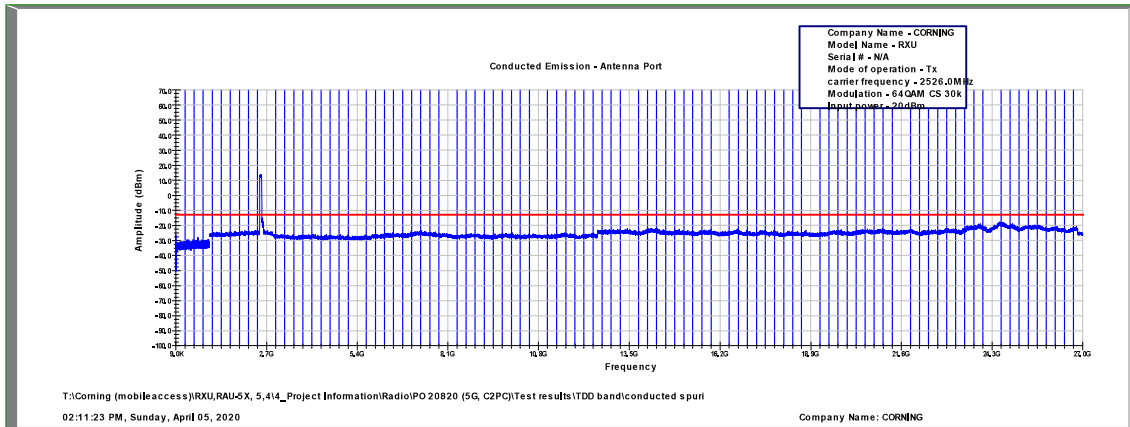
Figure 531: Spurious Emissions at Antenna Terminal 64QAM, 2526.0MHz, B.W. 60MHz, Sub Carrier 30kHz
