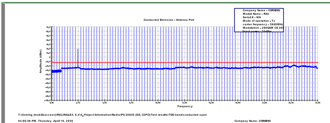
Figure 548: Spurious Emissions at Antenna Terminal 256QAM, 2685.0MHz, B.W. 10MHz, Sub Carrier 30kHz
