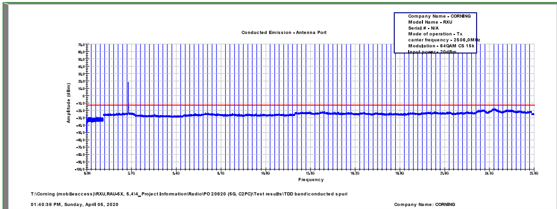
Figure 513: Spurious Emissions at Antenna Terminal 64QAM, 2506.0MHz, B.W. 20MHz, Sub Carrier 15kHz
