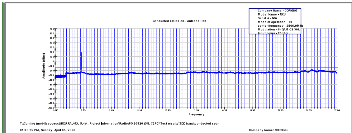
Figure 516: Spurious Emissions at Antenna Terminal 64QAM, 2506.0MHz, B.W. 20MHz, Sub Carrier 30kHz
