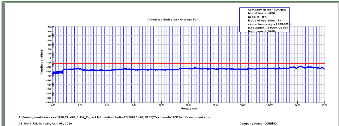
Figure 510: Spurious Emissions at Antenna Terminal 64QAM, 2503.5MHz, B.W. 15MHz, Sub Carrier 60kHz
