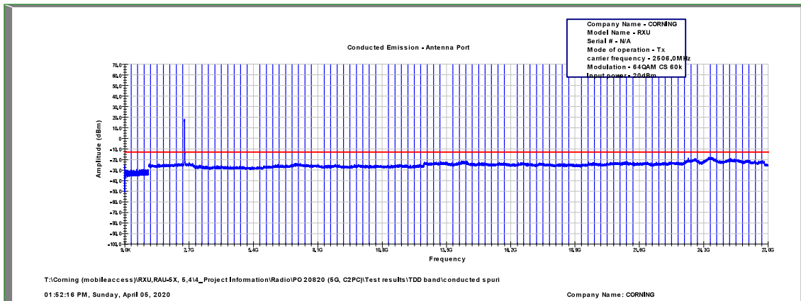
Figure 519: Spurious Emissions at Antenna Terminal 64QAM, 2506.0MHz, B.W. 20MHz, Sub Carrier 60kHz
