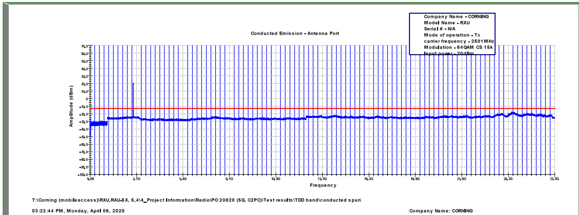
Figure 495: Spurious Emissions at Antenna Terminal 64QAM, 2501.00MHz, B.W. 10MHz, Sub Carrier 15kHz
