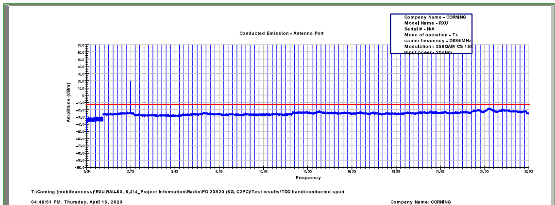
Figure 545: Spurious Emissions at Antenna Terminal 256QAM, 2685.0MHz, B.W. 10MHz, Sub Carrier 15kHz
