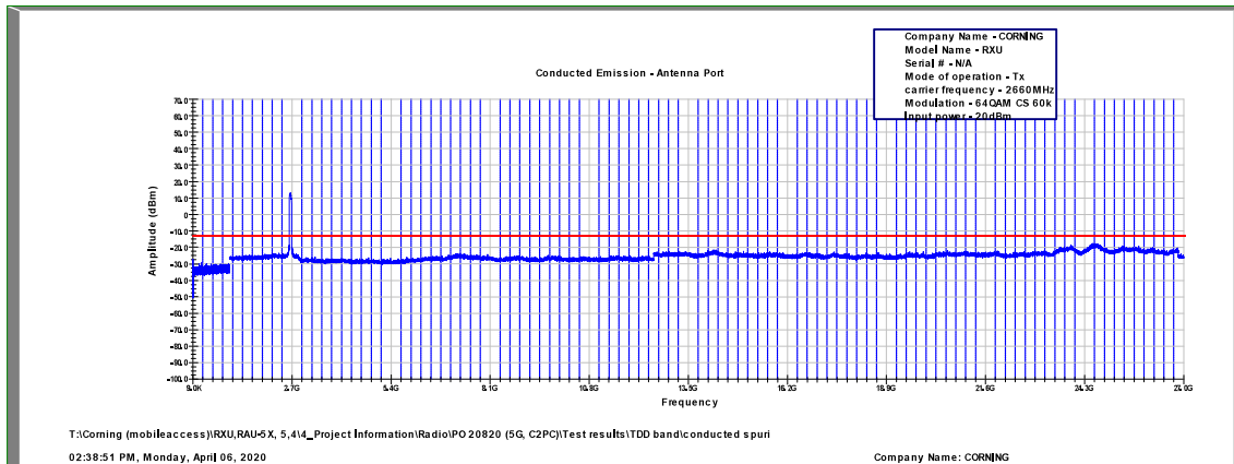
Figure 536: Spurious Emissions at Antenna Terminal 64QAM, 2660.0MHz, B.W. 60MHz, Sub Carrier 30kHz
