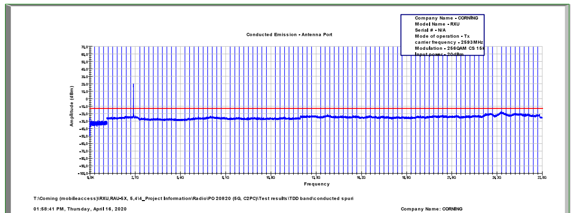
Figure 544: Spurious Emissions at Antenna Terminal 256QAM, 2593.0MHz, B.W. 10MHz, Sub Carrier 15kHz
