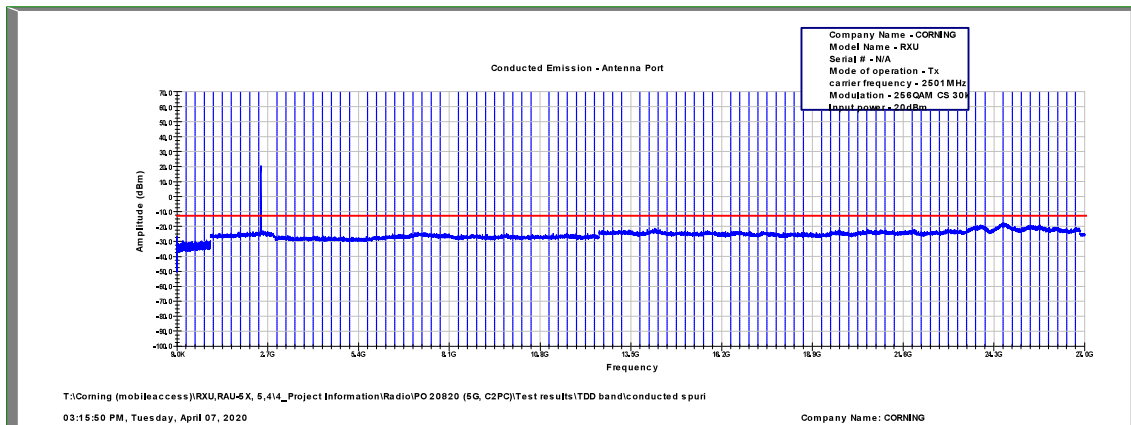
Figure 546: Spurious Emissions at Antenna Terminal 256QAM, 2501.0MHz, B.W. 10MHz, Sub Carrier 30kHz
