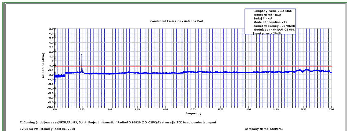
Figure 530: Spurious Emissions at Antenna Terminal 64QAM, 2670.0MHz, B.W. 40MHz, Sub Carrier 60kHz
