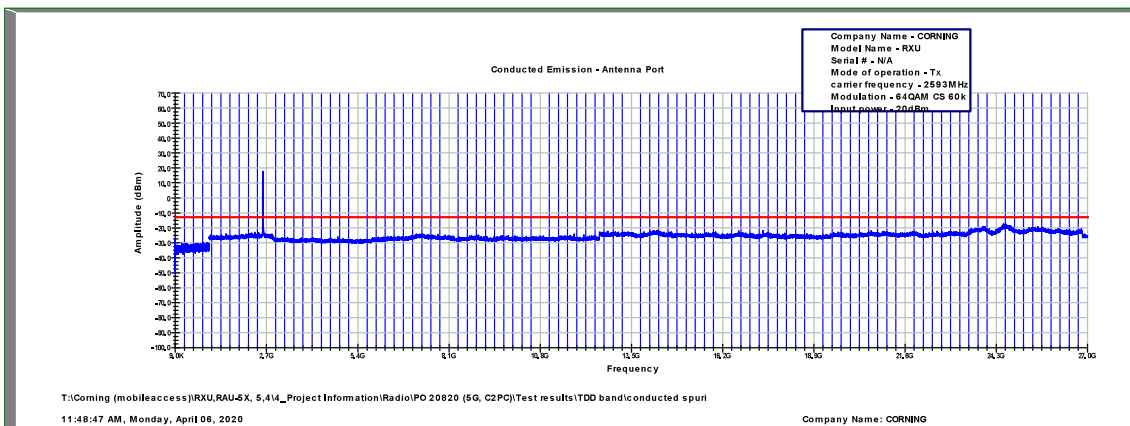
Figure 511: Spurious Emissions at Antenna Terminal 64QAM, 2593.0MHz, B.W. 15MHz, Sub Carrier 60kHz
