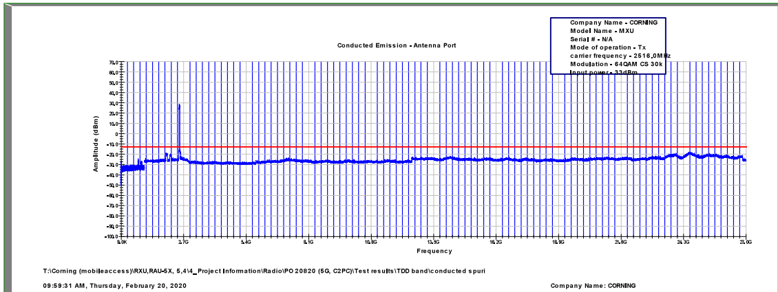
Figure 525: Spurious Emissions at Antenna Terminal 64QAM, 2516.0MHz, B.W. 40MHz, Sub Carrier 30kHz
