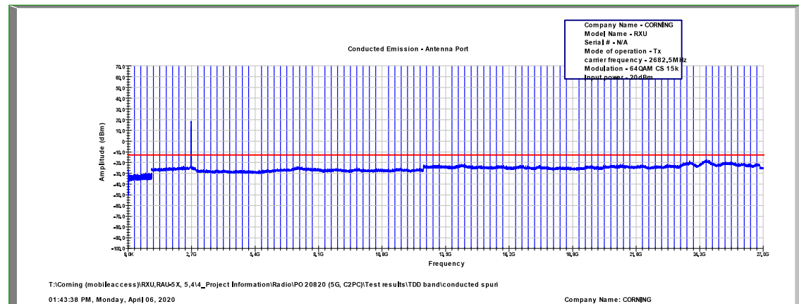
Figure 506: Spurious Emissions at Antenna Terminal 64QAM, 2682.5MHz, B.W. 15MHz, Sub Carrier 15kHz
