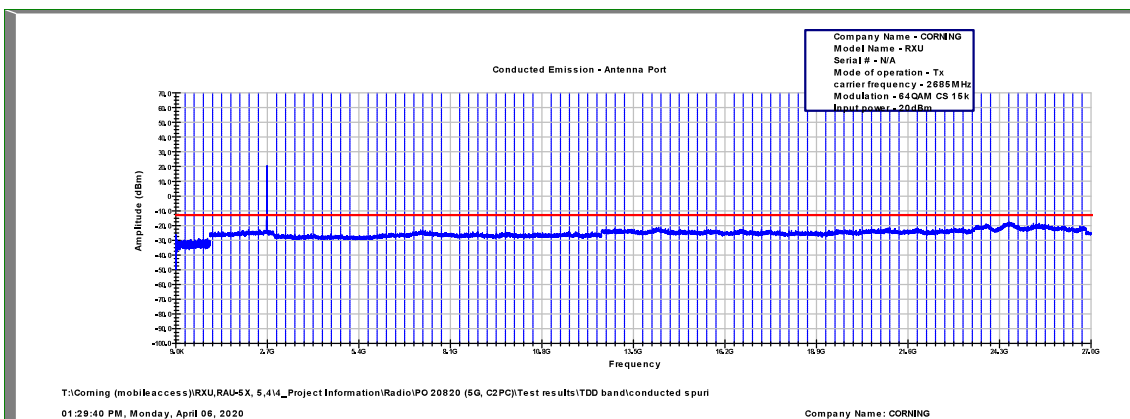
Figure 497: Spurious Emissions at Antenna Terminal 64QAM, 2685.0MHz, B.W. 10MHz, Sub Carrier 15kHz
