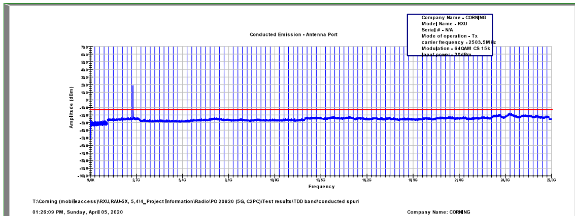
Figure 504: Spurious Emissions at Antenna Terminal 64QAM, 2503.5MHz, B.W. 15MHz, Sub Carrier 15kHz
