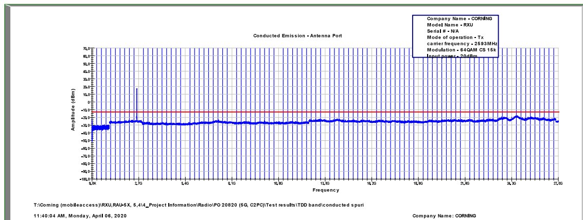
Figure 505: Spurious Emissions at Antenna Terminal 64QAM, 2593.0MHz, B.W. 15MHz, Sub Carrier 15kHz
