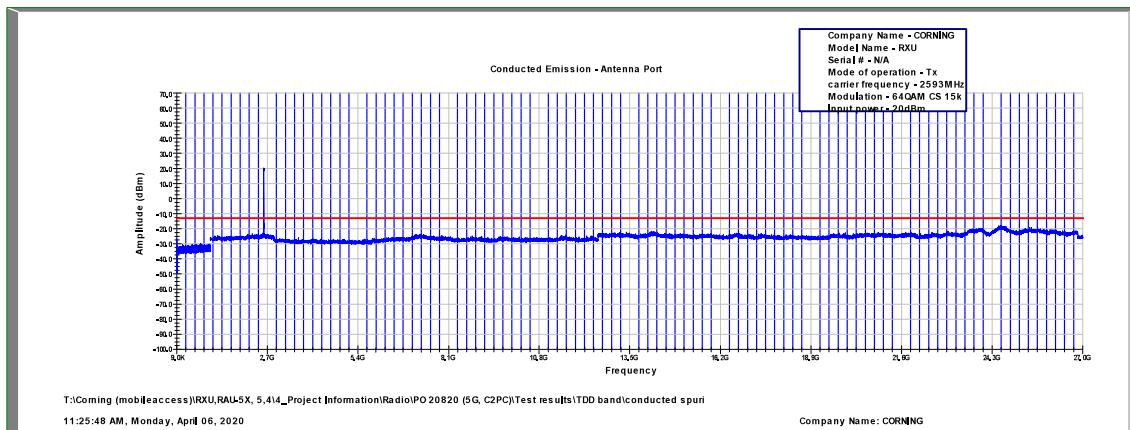
Figure 496: Spurious Emissions at Antenna Terminal 64QAM, 2593.0MHz, B.W. 10MHz, Sub Carrier 15kHz
