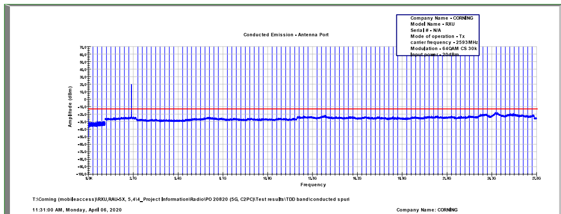
Figure 499: Spurious Emissions at Antenna Terminal 64QAM, 2593.0MHz, B.W. 10MHz, Sub Carrier 30kHz
