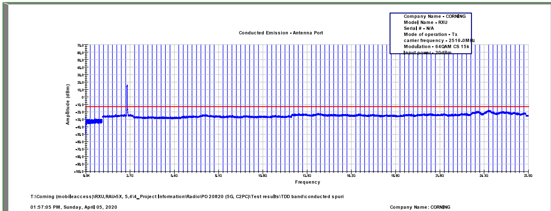
Figure 522: Spurious Emissions at Antenna Terminal 64QAM, 2516.0MHz, B.W. 40MHz, Sub Carrier 15kHz
