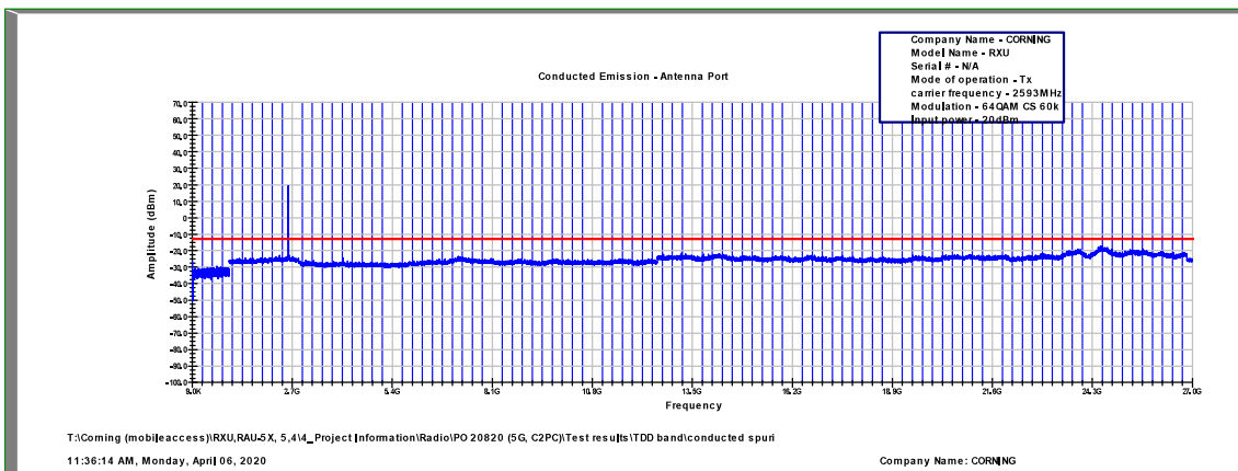
Figure 502: Spurious Emissions at Antenna Terminal 64QAM, 2593.0MHz, B.W. 10MHz, Sub Carrier 60kHz
