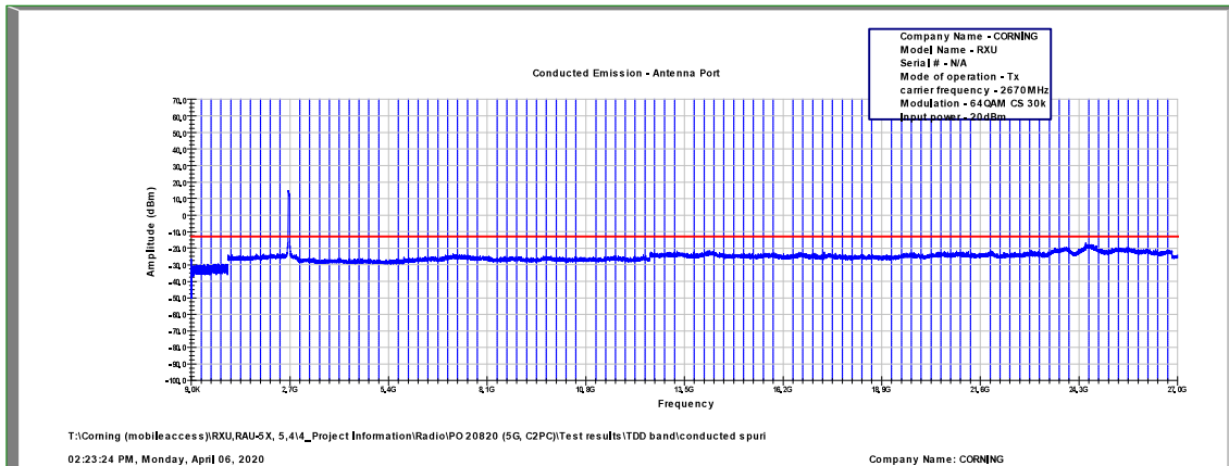
Figure 527: Spurious Emissions at Antenna Terminal 64QAM, 2670.0MHz, B.W. 40MHz, Sub Carrier 30kHz
