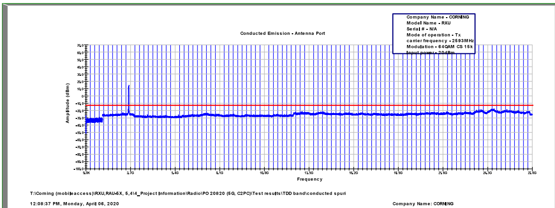
Figure 523: Spurious Emissions at Antenna Terminal 64QAM, 2593.0MHz, B.W. 40MHz, Sub Carrier 15kHz
