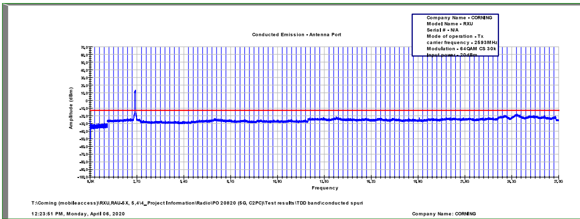
Figure 532: Spurious Emissions at Antenna Terminal 64QAM, 2593.0MHz, B.W. 60MHz, Sub Carrier 30kHz
