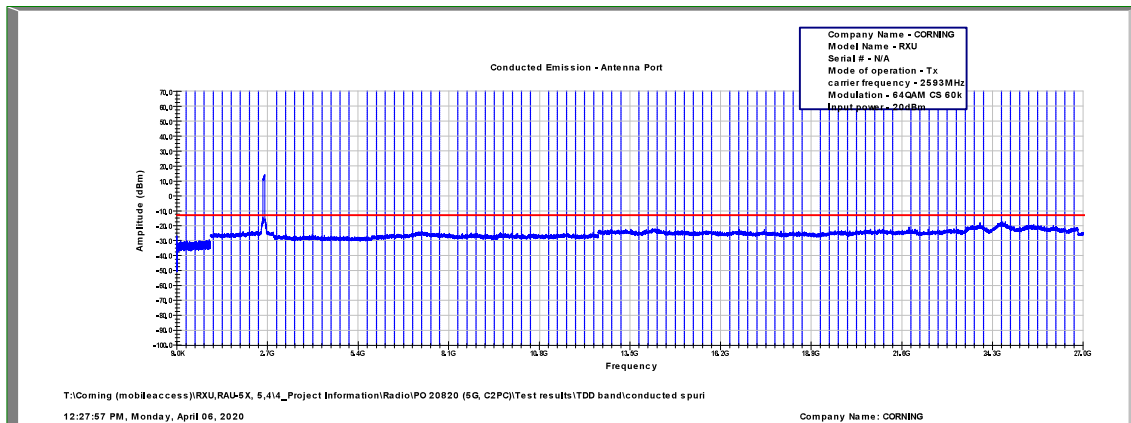
Figure 535: Spurious Emissions at Antenna Terminal 64QAM, 2593.0MHz, B.W. 60MHz, Sub Carrier 60kHz
