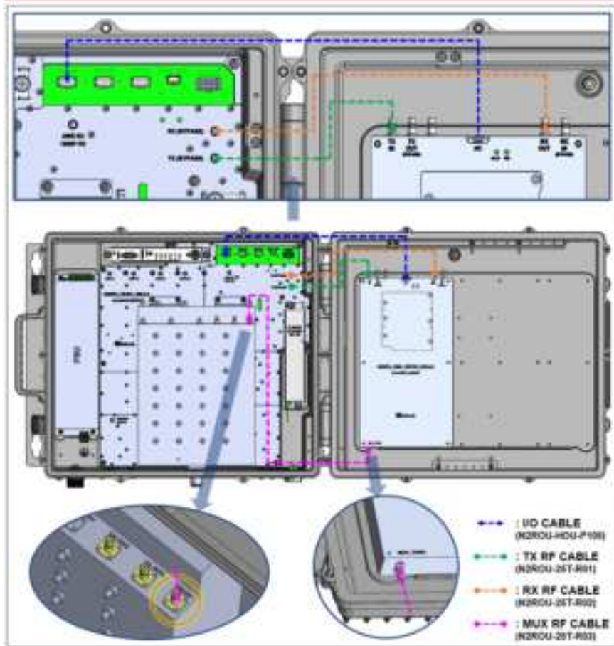
Figure 4.15 -N2RDU_2500_100TDD Cabling
