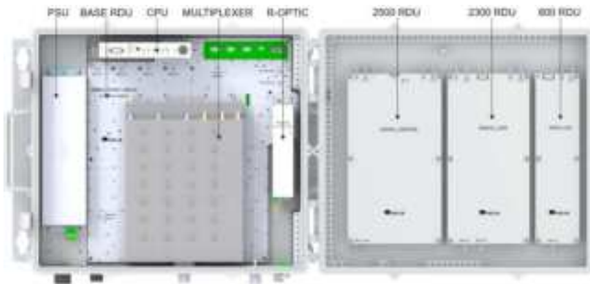
Figure 3.5 – Internal View of Remote Unit
