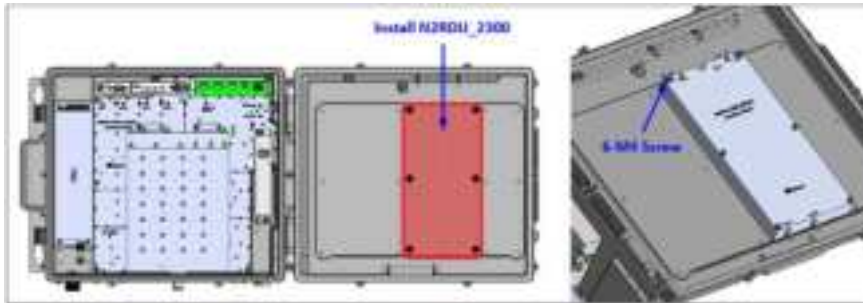
Figure 4.21 – Install N2RDU_2300
