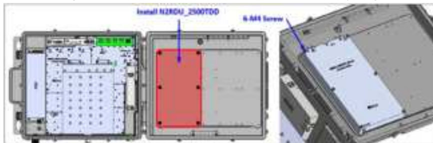
Figure 4.12 – Install N2RDU_2500TDD
