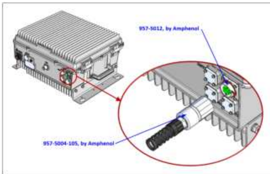
Figure 4.10 –Optical Connector
