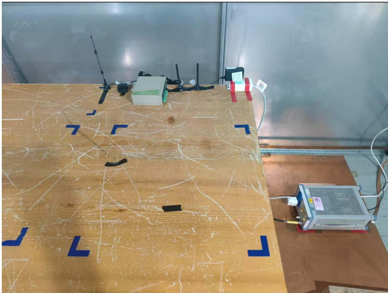
RF Conducted Test setup (AC Power line)
