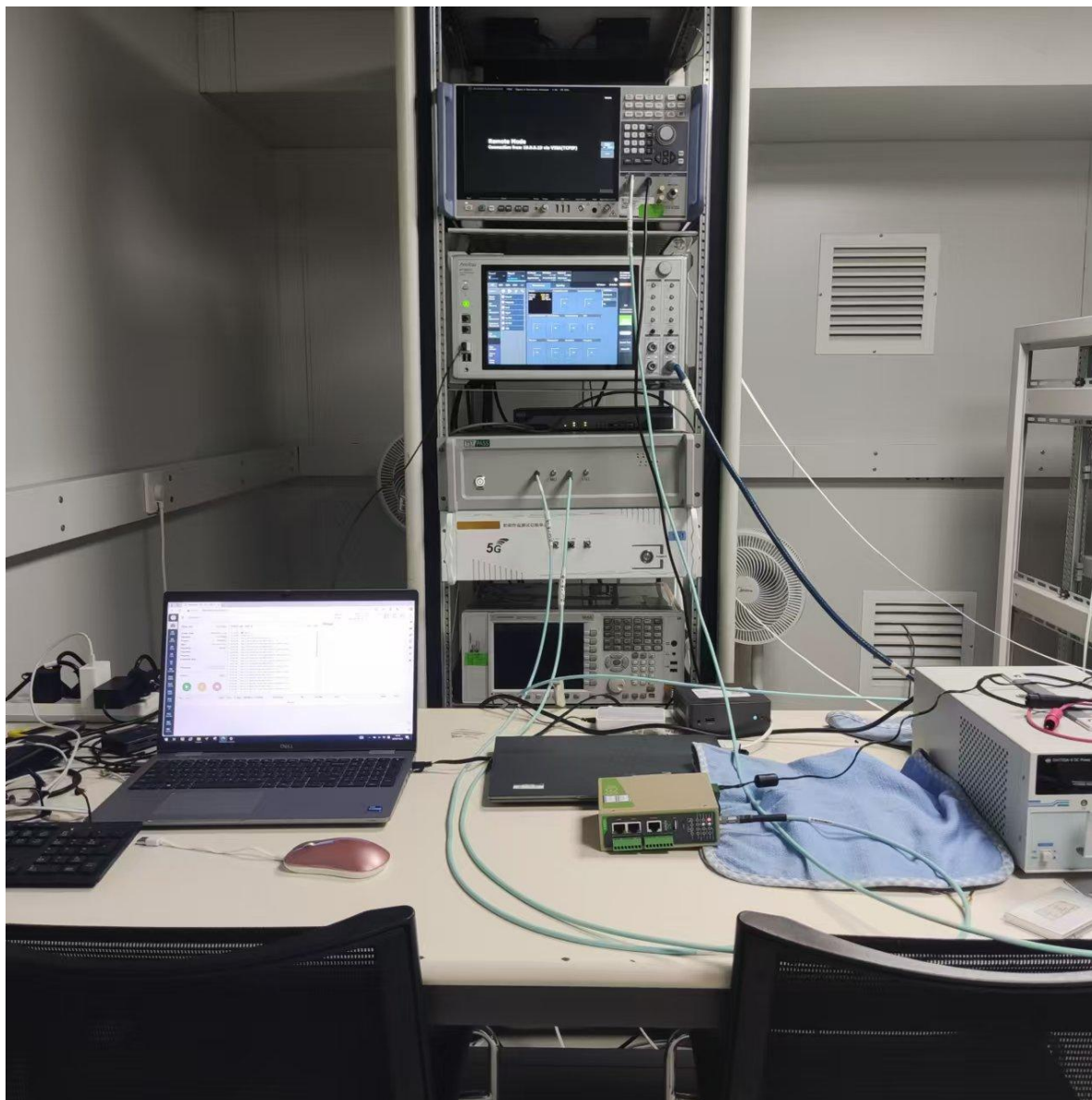
RF Conducted Test setup (LTE)
