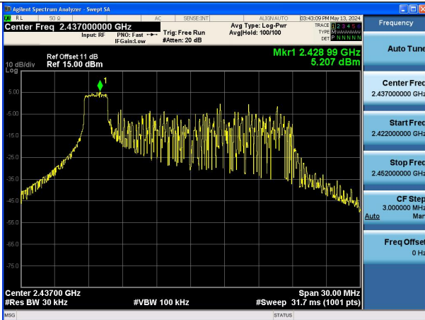
Mode:802.11ax HE20 Tone:26T Frequency:2437MHz Ant:Chain1
