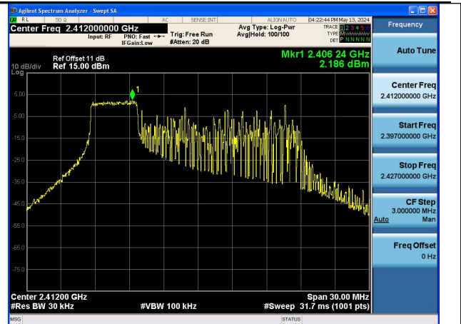
Mode:802.11ax HE20 Tone:52T Frequency:2412MHz Ant:Chain1
