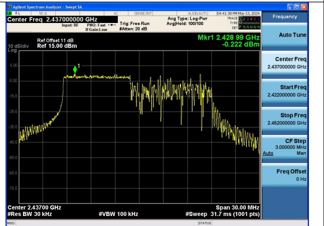
Mode:802.11ax HE20 Tone:106T Frequency:2437MHz Ant:Chain0
