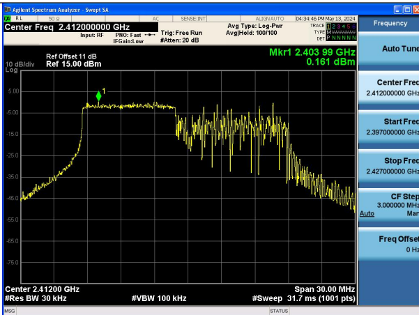
Mode:802.11ax HE20 Tone:106T Frequency:2412MHz Ant:Chain0
