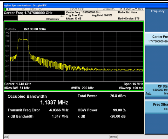
Band4-15MHz-QPSK-20325-6-0-Low-1.1337-1.347-PASS
