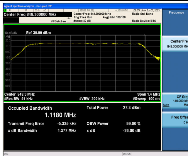
Band5-1.4MHz-QPSK-20643-6-0-Low-1.1180-1.377-PASS
