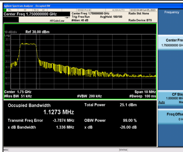
Band4-10MHz-QPSK-20350-6-0-Low-1.1273-1.336-PASS
