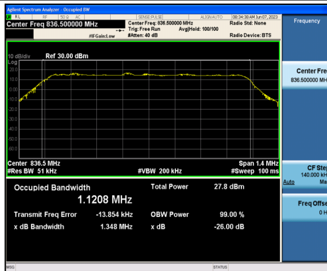
Band5-1.4MHz-QPSK-20525-6-0-Low-1.1208-1.348-PASS
