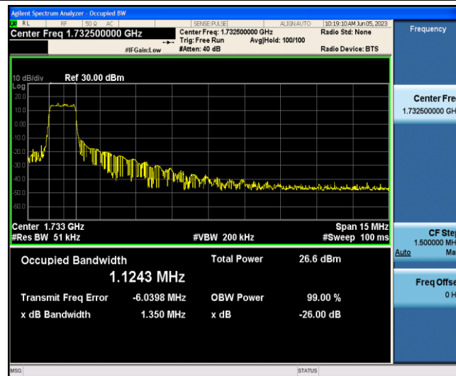
Band4-15MHz-QPSK-20175-6-0-Low-1.1243-1.350-PASS
