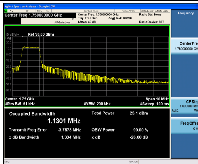
Band4-10MHz-16QAM-20350-6-0-Low-1.1301-1.334-PASS
