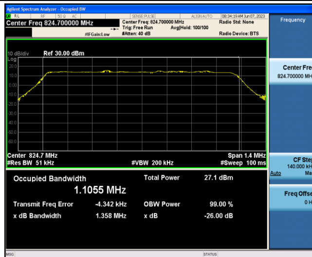
Band5-1.4MHz-16QAM-20407-6-0-Low-1.1055-1.358-PASS
