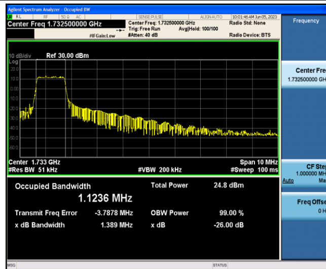
Band4-10MHz-16QAM-20175-6-0-Low-1.1236-1.389-PASS
