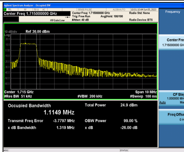
Band4-10MHz-16QAM-20000-6-0-Low-1.1149-1.319-PASS
