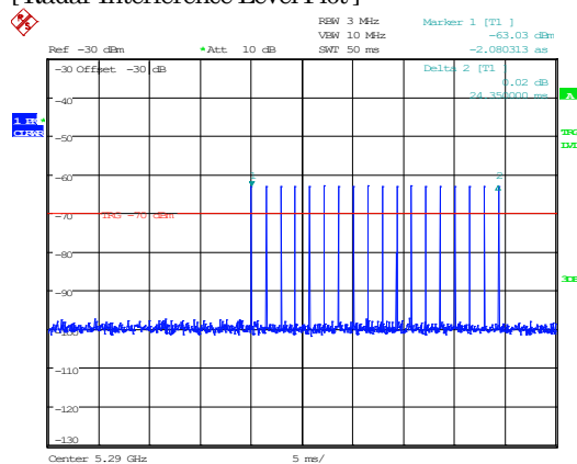
[ Radar Interference Level Plot ]
