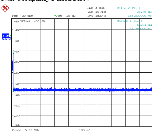
[ Non-Occupancy Period Plot ]
