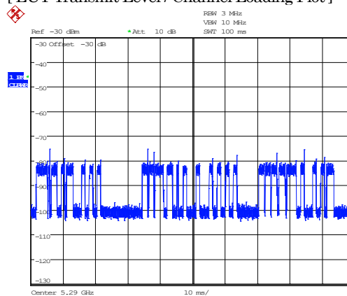
[ EUT Transmit Level / Channel Loading Plot ]
