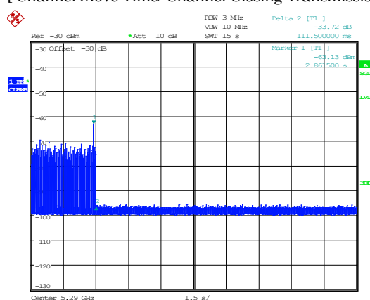
[ Channel Move Time/ Channel Closing Transmission Time ]
