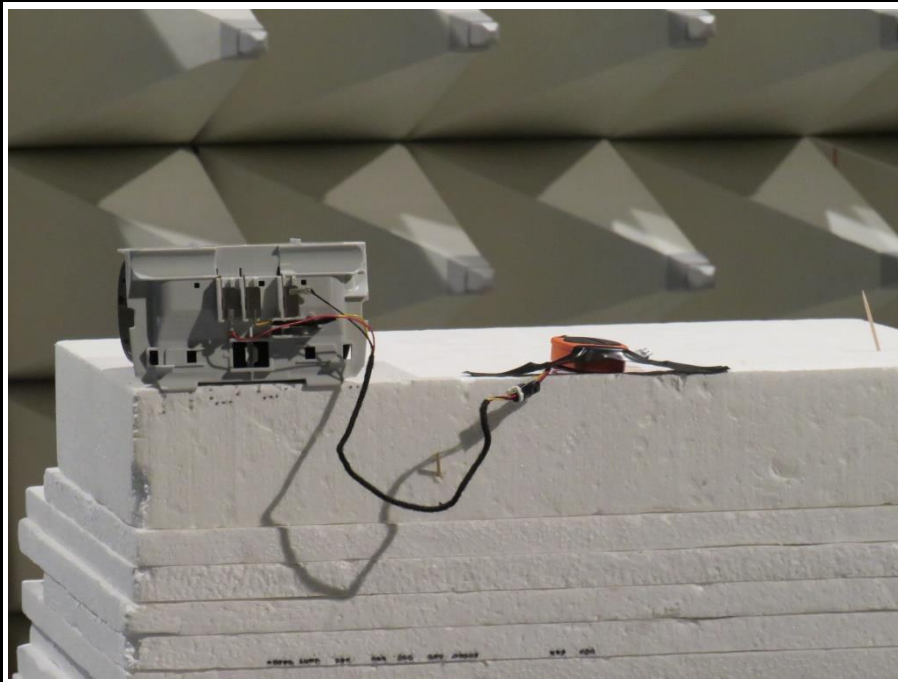
Test Setup Near View Above 1GHz - EUT horizontal
