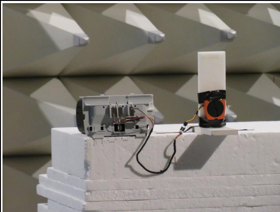
Test Setup Near View Above 1GHz - EUT vertical
