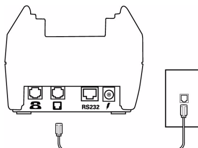
Figure 26 Direct Connection
