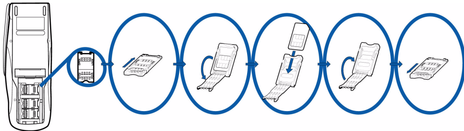
Figure 10 MSAM Card Installation
