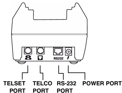
Figure 25 Omni 3600 Base Connection Ports
