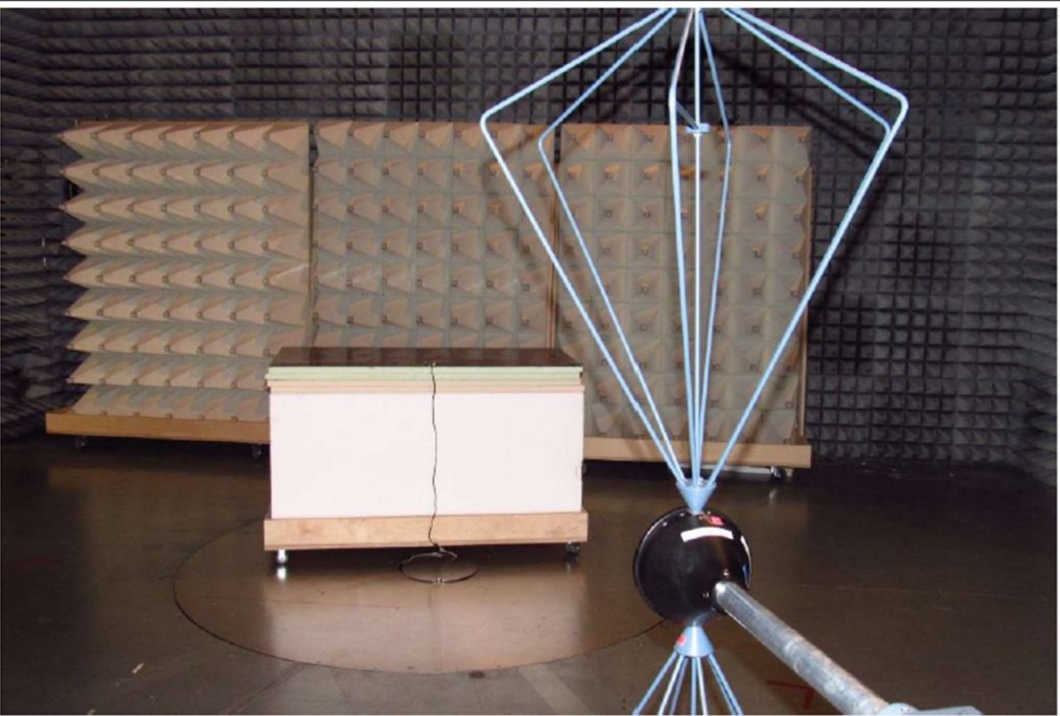
Radiated Setup - View B
