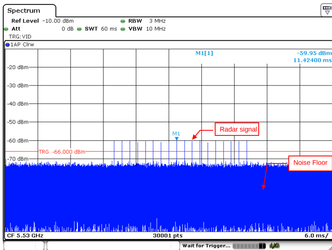
Radar Signal 0
