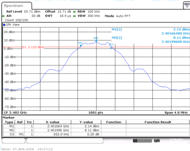
BLE_1M-Ant1-2402-PASS
