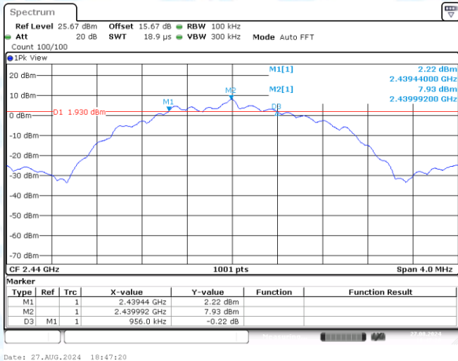
BLE_2M-Ant1-2440-PASS
