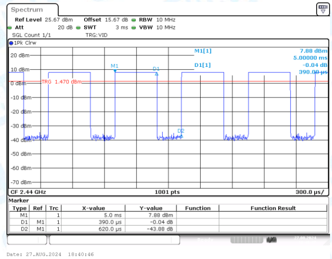
NTNV-BLE_1M-Ant1-2440
