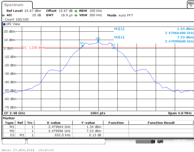
BLE_1M-Ant1-2480-PASS
