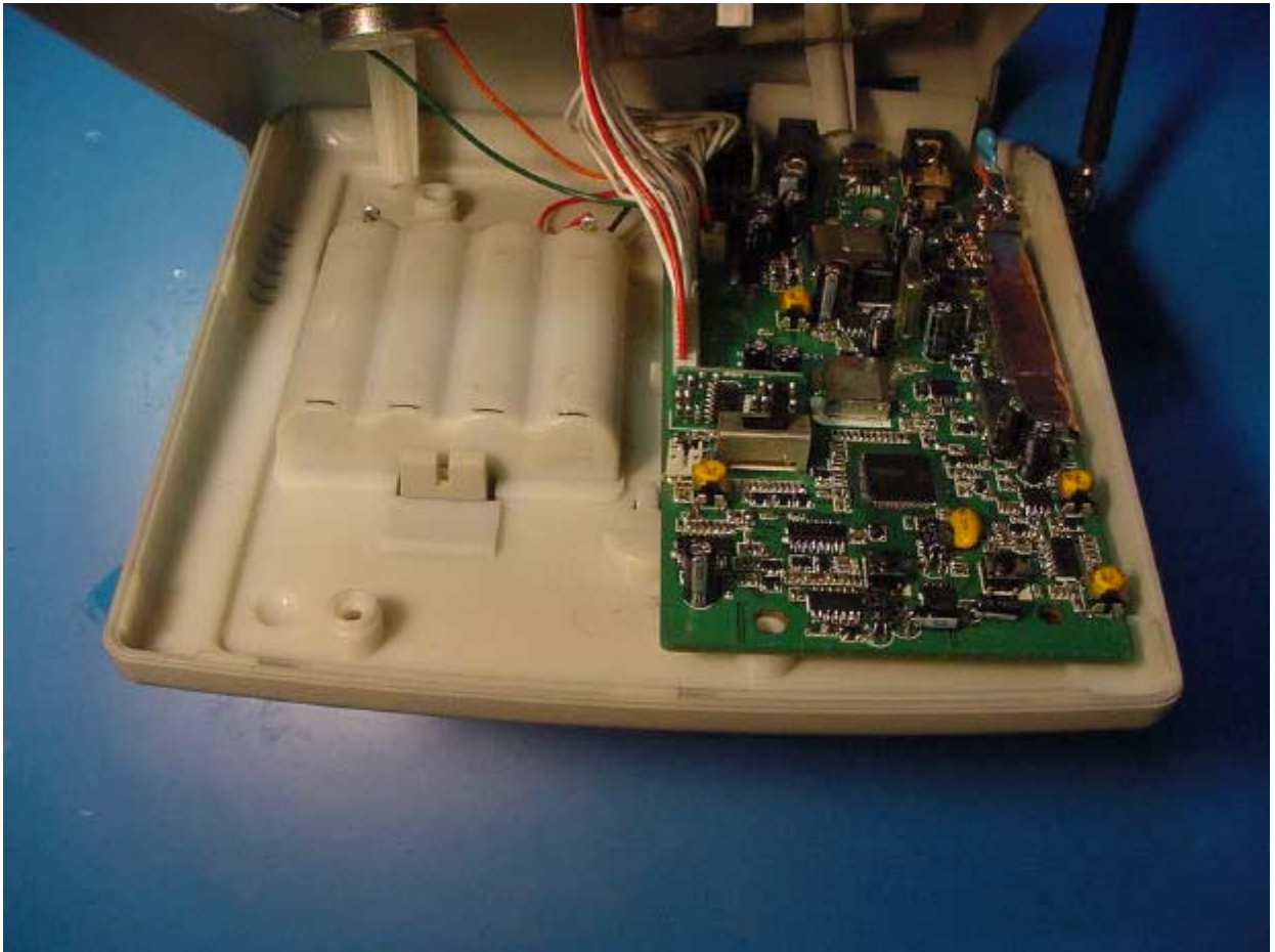
Inside bottom of case with main PCB
