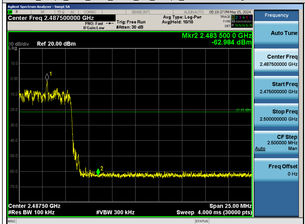
Test Graph EDR HOP ANT1 NA 3Mbps Higher Band Edge Emissions
