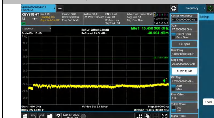
Band2-10MHz-QPSK-18650-1RB#0-3000~20000-PASS
