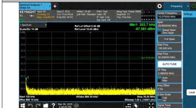
Band2-10MHz-QPSK-19150-1RB#49-0.15~30-PASS
