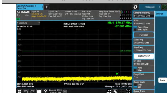
Band2-10MHz-QPSK-18650-1RB#0-30~1000-PASS
