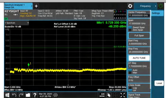
Band2-1.4MHz-QPSK-19193-1RB#5-3000~20000-PASS
