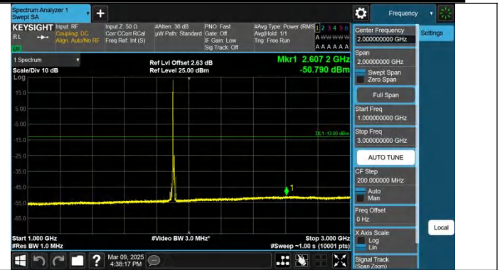
Band2-10MHz-QPSK-19150-1RB#0-1000~3000-PASS
