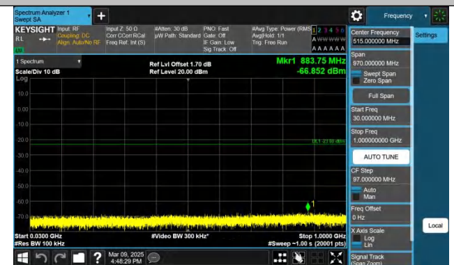
Band2-15MHz-QPSK-19125-1RB#74-30~1000-PASS
