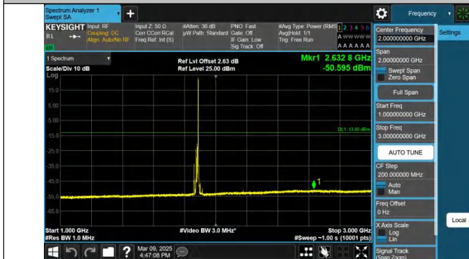
Band2-15MHz-QPSK-18900-1RB#74-1000~3000-PASS
