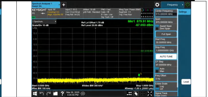
Band2-10MHz-QPSK-18650-1RB#49-30~1000-PASS
