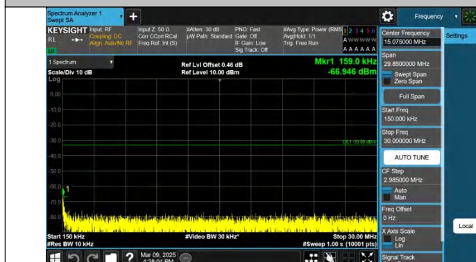
Band2-5MHz-QPSK-19175-1RB#24-0.15~30-PASS
