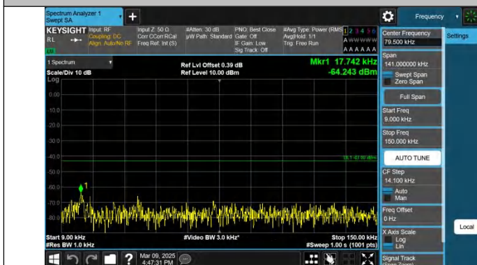
Band2-15MHz-QPSK-19125-1RB#0-0.009~0.15-PASS
