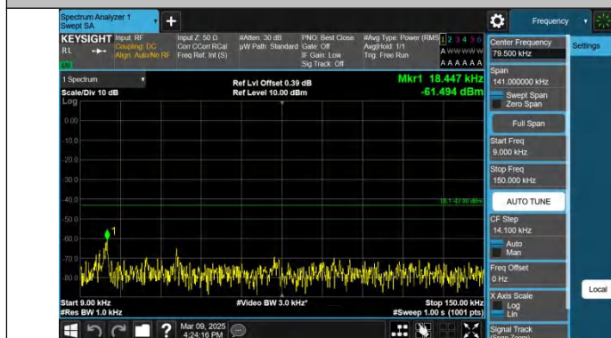
Band2-5MHz-QPSK-18625-1RB#0-0.009~0.15-PASS
