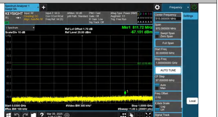
Band2-5MHz-QPSK-19175-1RB#24-30~1000-PASS
