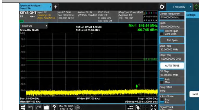
Band2-20MHz-QPSK-19100-1RB#0-30~1000-PASS
