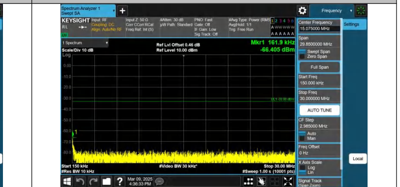
Band2-10MHz-QPSK-18900-1RB#0-0.15~30-PASS
