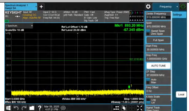
Band2-1.4MHz-QPSK-19193-1RB#5-30~1000-PASS
