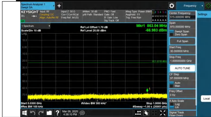
Band2-10MHz-QPSK-19150-1RB#0-30~1000-PASS
