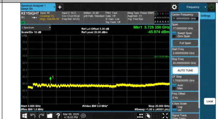
Band2-3MHz-QPSK-19185-1RB#14-3000~20000-PASS
