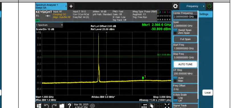
Band2-10MHz-QPSK-18900-1RB#0-1000~3000-PASS
