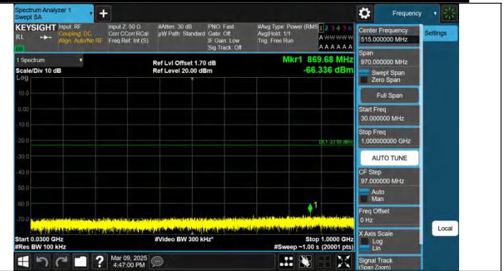
Band2-15MHz-QPSK-18900-1RB#74-30~1000-PASS
