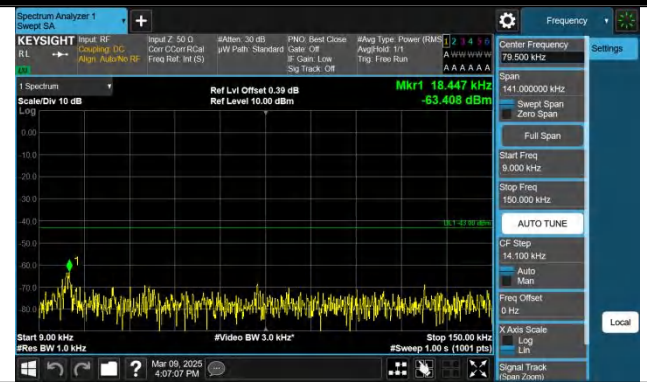
Band2-1.4MHz-QPSK-19193-1RB#5-0.009~0.15-PASS
