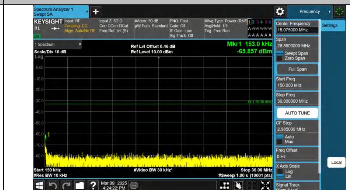
Band2-5MHz-QPSK-18625-1RB#0-0.15~30-PASS
