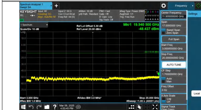
Band2-20MHz-QPSK-18700-1RB#0-3000~20000-PASS
