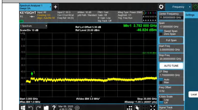
Band2-20MHz-QPSK-19100-1RB#0-3000~20000-PASS
