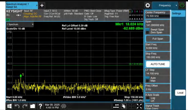
Band2-15MHz-QPSK-19125-1RB#74-0.009~0.15-PASS
