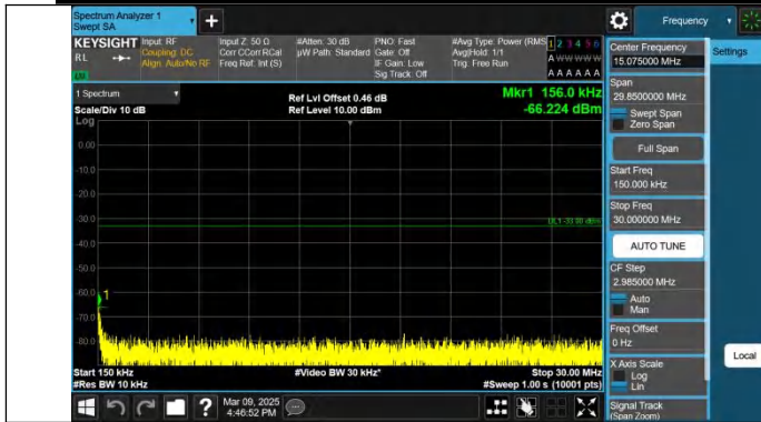
Band2-15MHz-QPSK-18900-1RB#74-0.15~30-PASS
