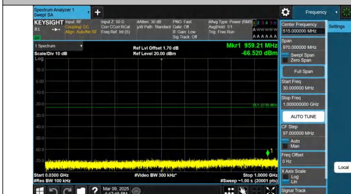
Band2-15MHz-QPSK-19125-1RB#0-30~1000-PASS
