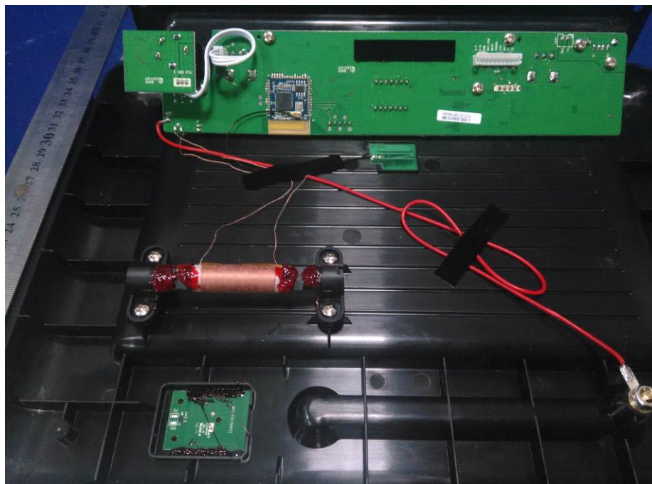
NFC Antenna (RX Only)
