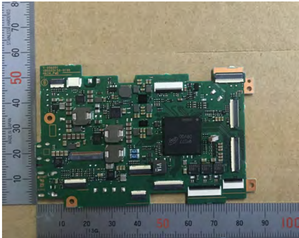
PWB MAIN_A
