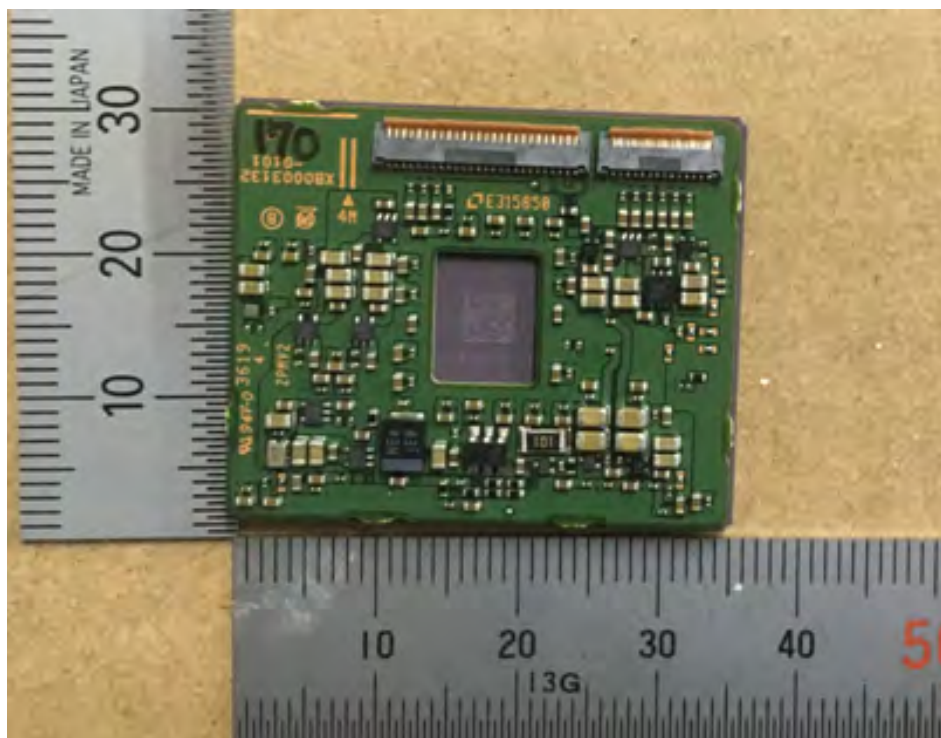
PWB CMOS_B
