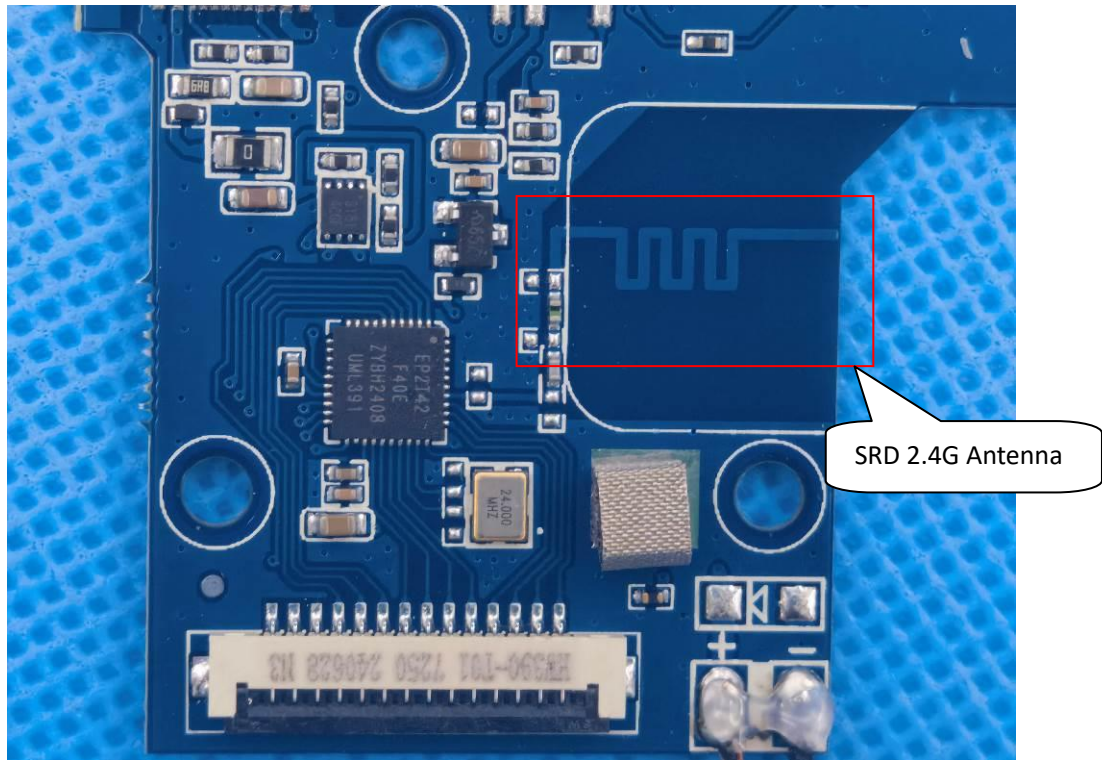
INTERNAL VIEW OF EUT (FIGURE 4)
