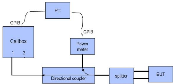
(b) Appendix A – Test Setup Photo 5
