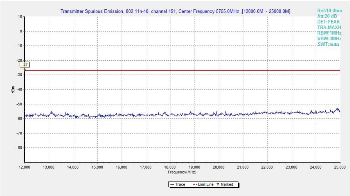
Fig. 35 Conducted Spurious Emission (802.11n40, Ch151 , 12 GHz ~ 25 GHz)
