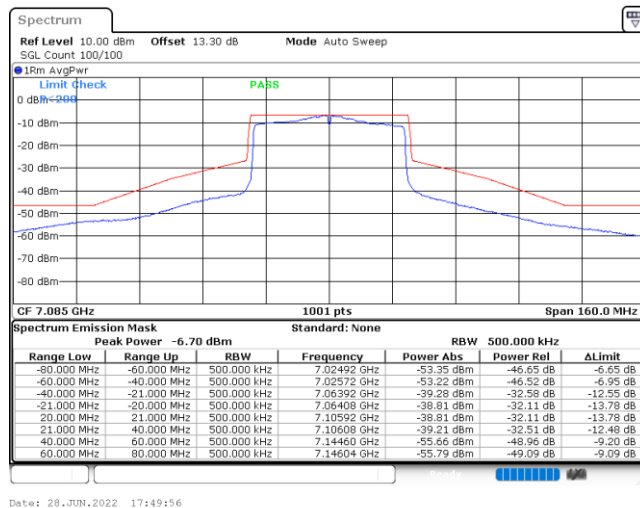
Plot on Channel 7085MHz
