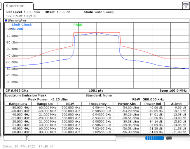
Plot on Channel 6965MHz
