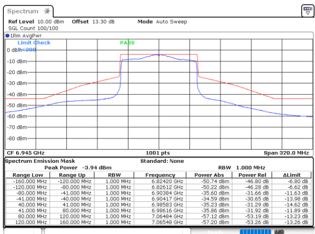
Plot on Channel 6945MHz
